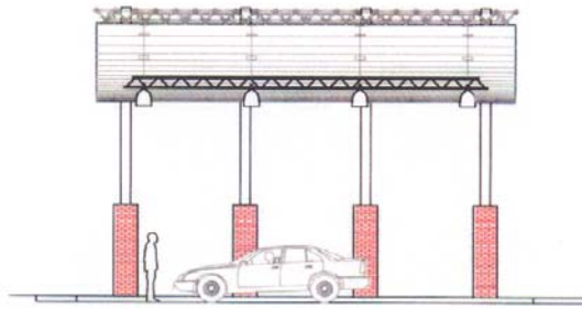
Figure 3. Longitudinal Section of Vehicle Inspection Canopy Example
