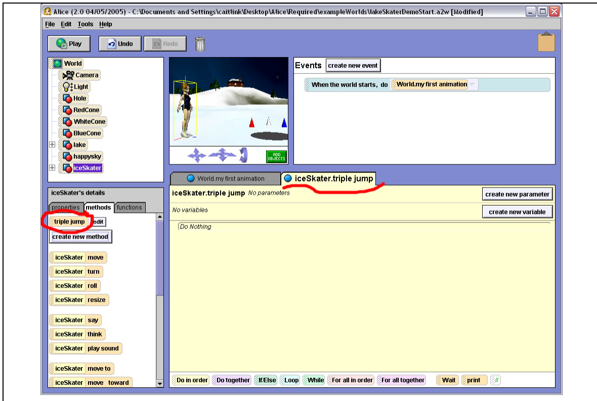
Figure 2.11: The interface after the user has created a “triple jump” method for the iceSkater. Alice has created a tile the user can drag into their program to call “triple jump” and opened a method editor where the user can define the behavior for “triple jump.”
