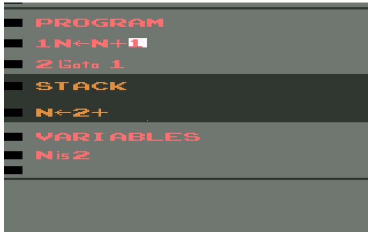
Figure 11.17: A simple program in Atari 2600 BASIC. The areas of the screen update to show the current position and state of the program.
