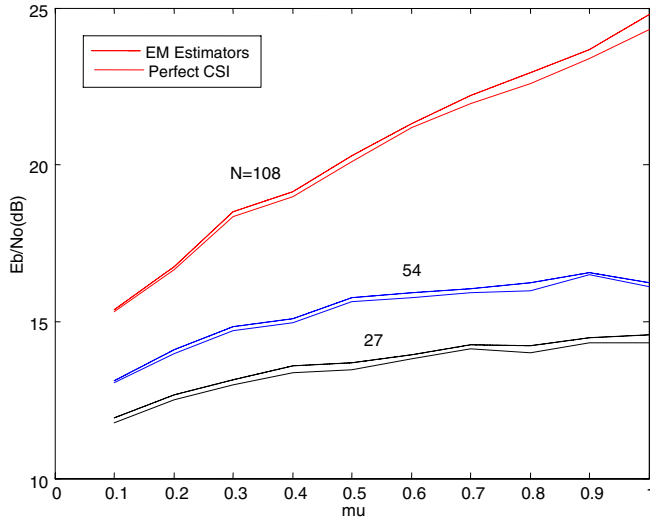
Fig. 6. Minimum required \mathcal{E}_b/N_o of frequency-hopping system with quaternary CPFSK, h = 0.46 , Rayleigh fading, partial-band interference, \mathcal{E}_b/I_{t0} = 13 dB, and bit error probability = 10^{-3} . N is the number of code symbols per hop.
