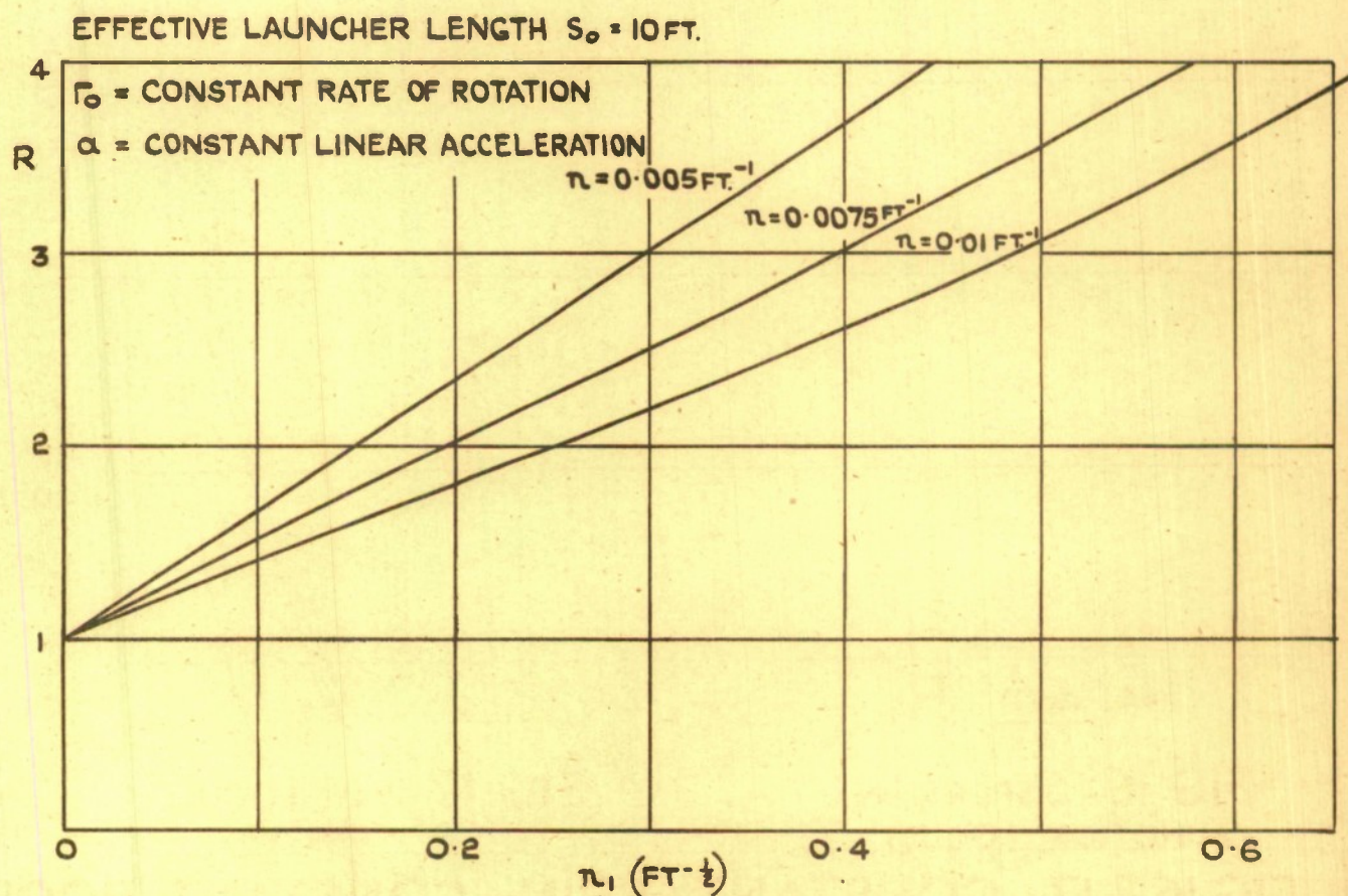
FIG.19. FACTOR R BY WHICH DISPERSION OF UNSPUN ROUND IS REDUCED AGAINST n_1 = \sqrt{\frac{2}{a}} \tau_0
