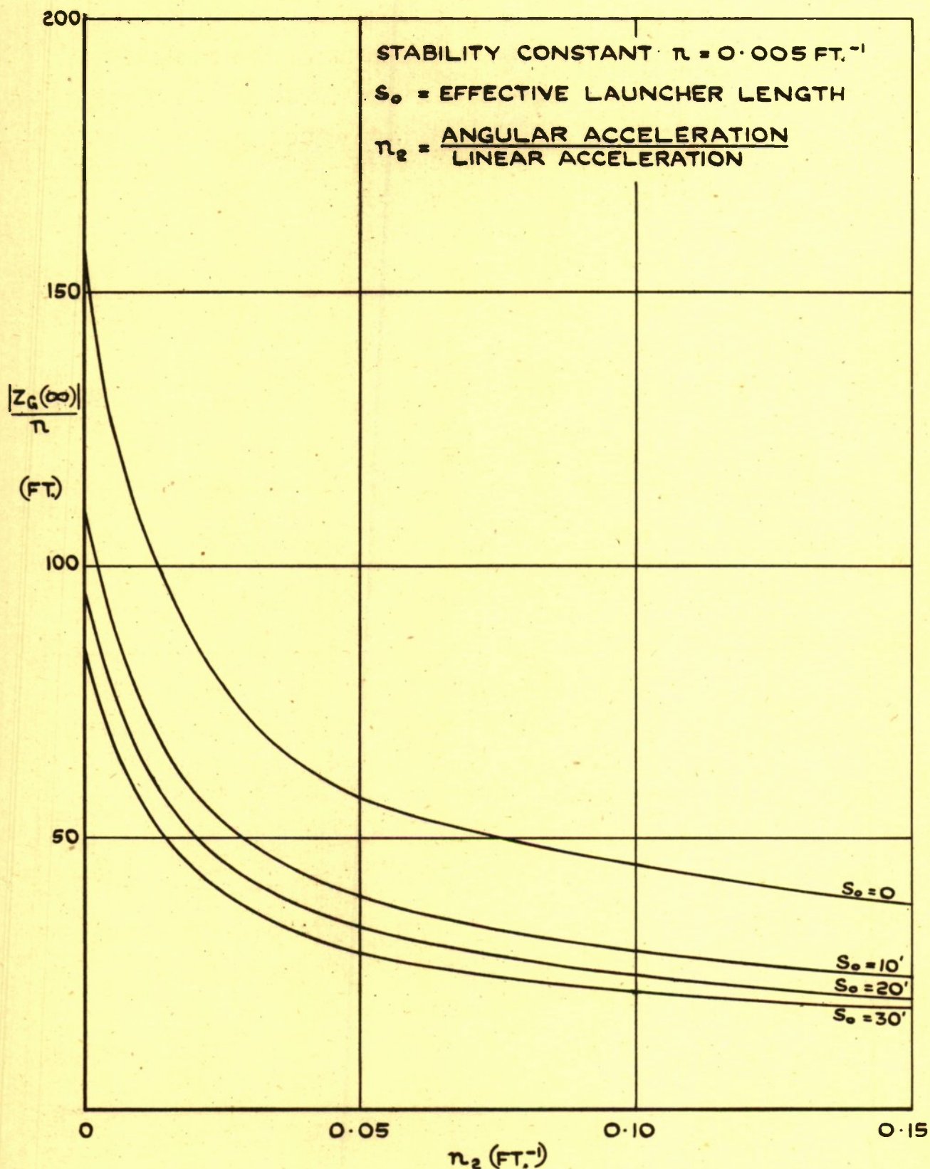
FIG.6 DISPERSION FUNCTIONS FOR BOOST DESTABILISING COUPLE. ZERO LAUNCHING SPIN. CONSTANT ANGULAR ACCELERATION.
