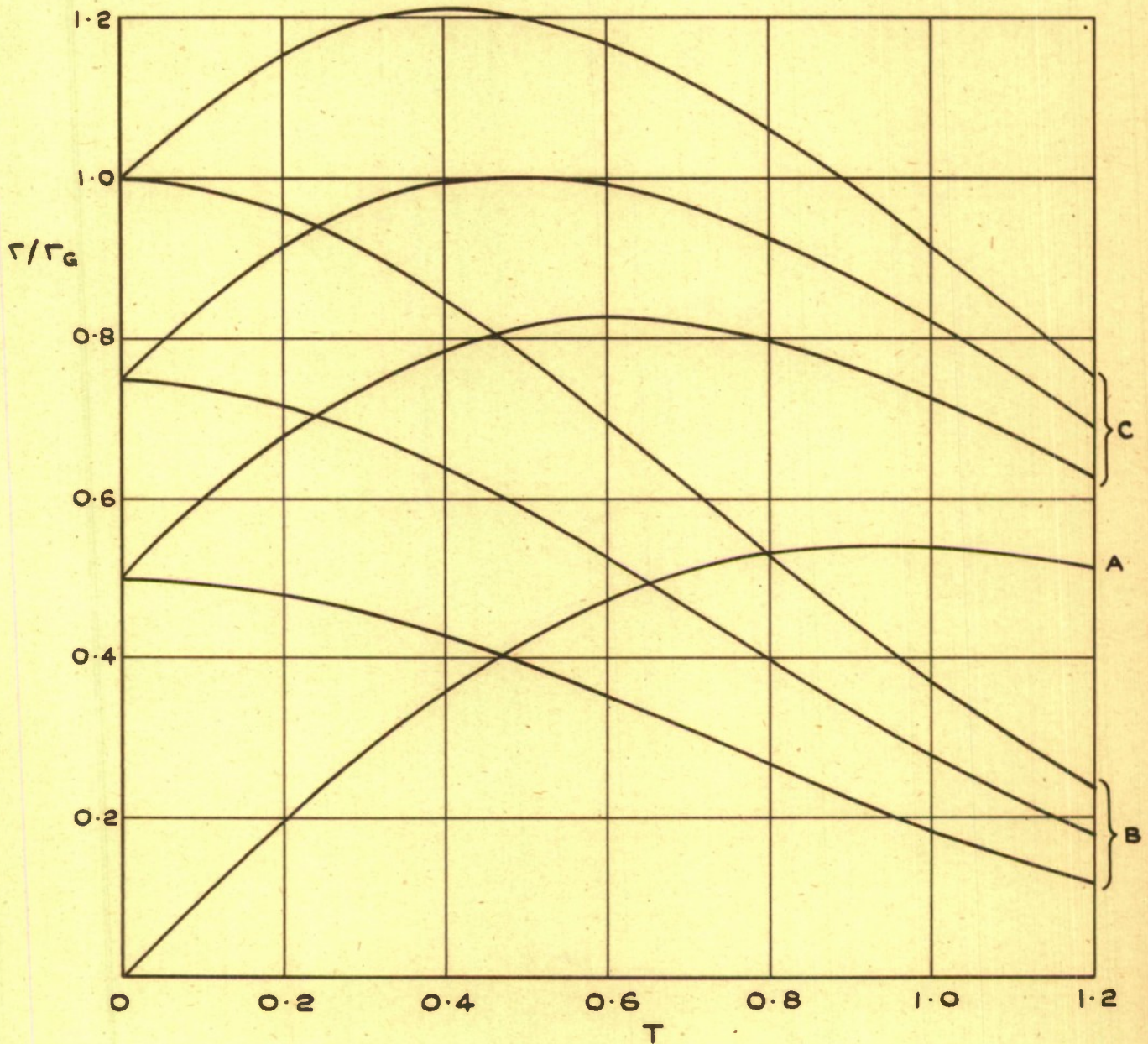
FIG. 1 SPIN-FORMS. (PLOTTED NON-DIMENSIONALLY)
