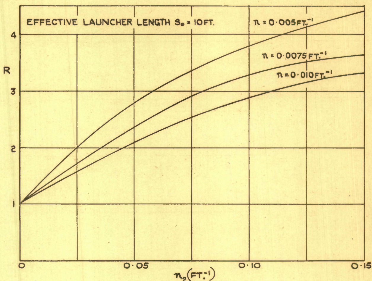
FIG.18. FACTOR R BY WHICH DISPERSION OF UNSPUN ROUND IS REDUCED AGAINST n_2 = \frac{\text{ANGULAR ACCELERATION}}{\text{LINEAR ACCELERATION}} . ZERO LAUNCHING SPIN.
