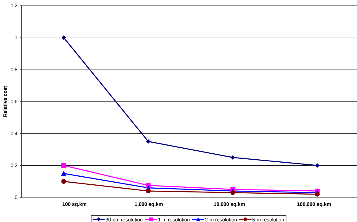
Figure 68. Estimation of typical cost of LIDAR data and DTM based on the size of the collection area and required DTM resolution.
