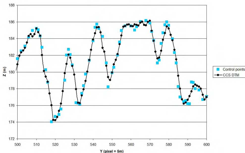
Figure 50. CCS DTM and control points for 500 m (= 100 pixels) of line No. 728. Blue squares are control points, black circles are DTM. Bias of CCS DTM from 2186 control points is +3.1 cm.
