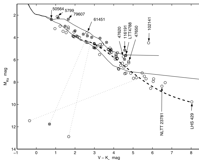
FIG. 1.—Joint color-absolute magnitude diagram of CPM pairs in M_{K_s} vs. V - K_s axes. The ZAMS and 16 Myr isochrones are drawn from (Siess et al. 2000), both for Z = 0.001 . The three white dwarfs of our sample are connected with their M dwarf companions by dotted straight lines. The thicker dashed line indicates the empirical main sequence for field dwarfs from Henry et al. (2004). Known unresolved binary companions of all kinds are marked with crosses inscribed in circles.
