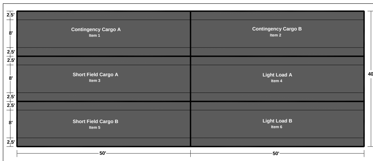
Figure 2. Plan view of test section.
