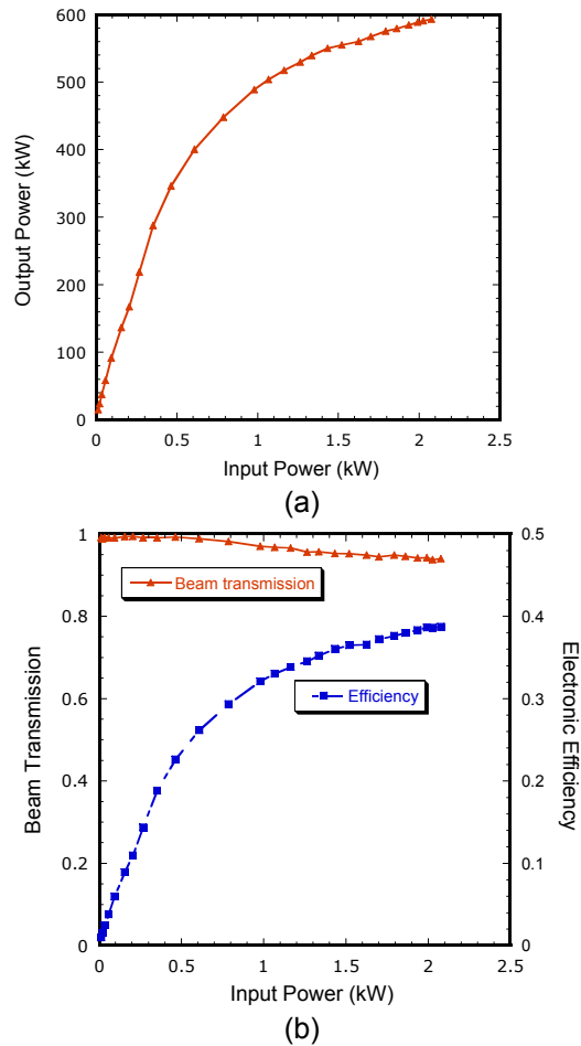
Figure 2: (a) Measured MBK2 output power, and (b) beam transmission and electronic efficiency, versus input power ( f = 3.15 GHz).
