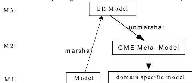
Figure 1. Marshaling and unmarshaling models
