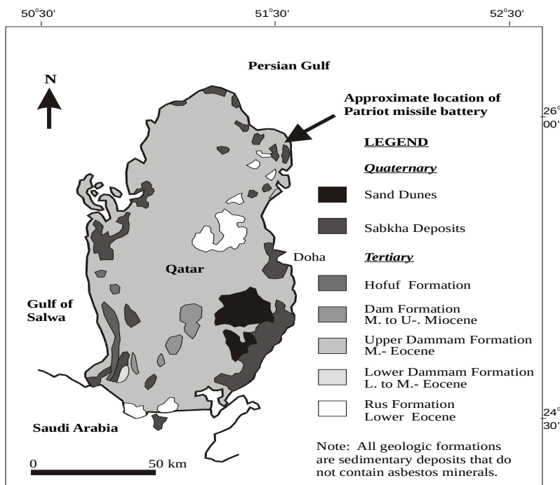
Fig 1. Geologic Map of Qatar. 6 (Note: No asbestos occurs in these deposits)
