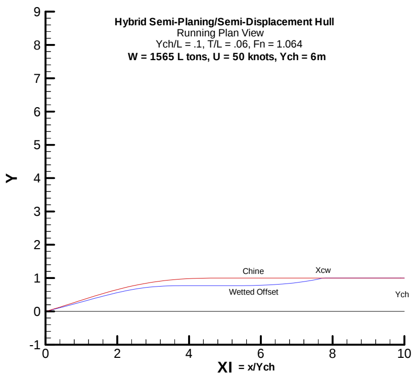
Fig 2 : Running Half-Breadth Plan of Hybrid Semihull
