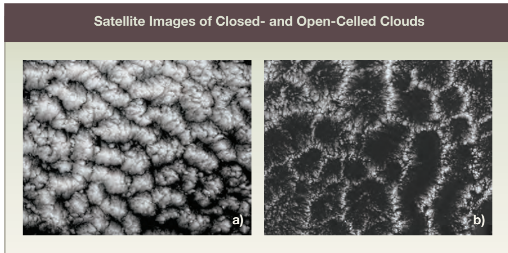
Figure 4: Satellite Images of Closed- and Open-Celled Clouds. 9 The width of the closed-cell (a) and open-cell (b) clouds images is approximately 200 km and 280 km, respectively.
