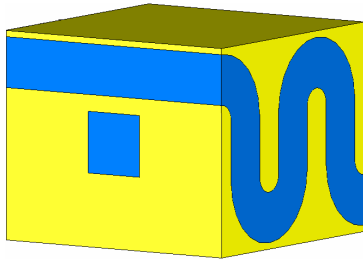
Fig. 1. Section of folded-waveguide slow-wave circuit. Electron beam passing through square aperture interacts with electromagnetic wave passing through serpentine waveguide.
