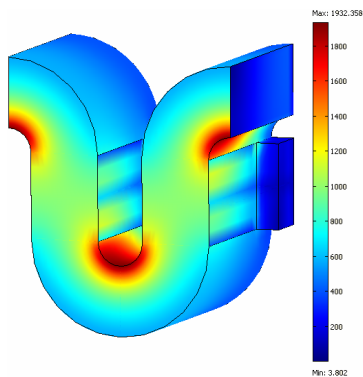
Fig. 2. Computed surface current densities for half of a geometric period of folded-waveguide slow-wave circuit.
