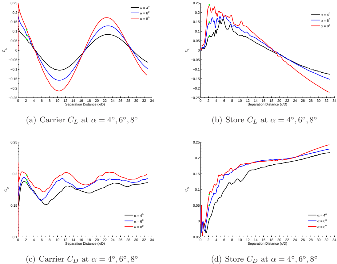
Figure 4.24: Carrier/Store Lift/Drag Coefficients at \alpha = 4^\circ, 6^\circ, 8^\circ
