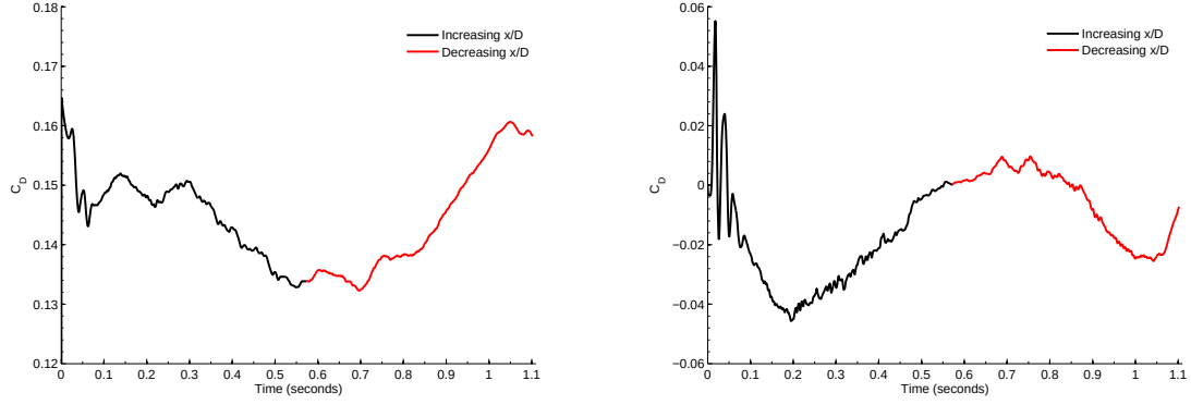
(a) Carrier C_D for Failed Separation at \alpha = 0^\circ (b) Store C_D for Failed Separation at \alpha = 0^\circ
