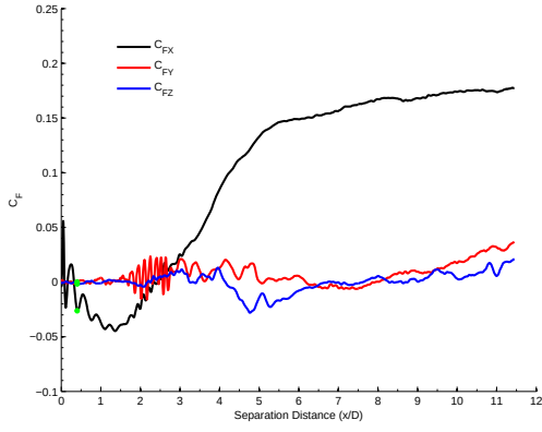
(a) Store C_F at \gamma = 0^\circ
