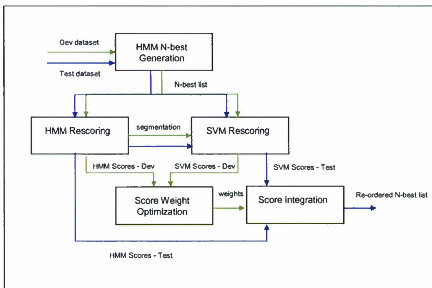
Figure 4: N-best rescoring procedure for using stochastic segment models.
