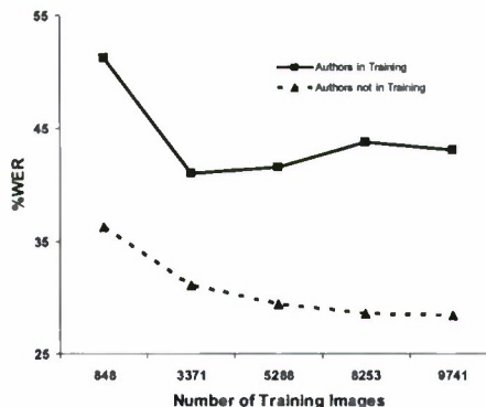
Figure 3: Comparison of recognition performance with amounts of training data.
