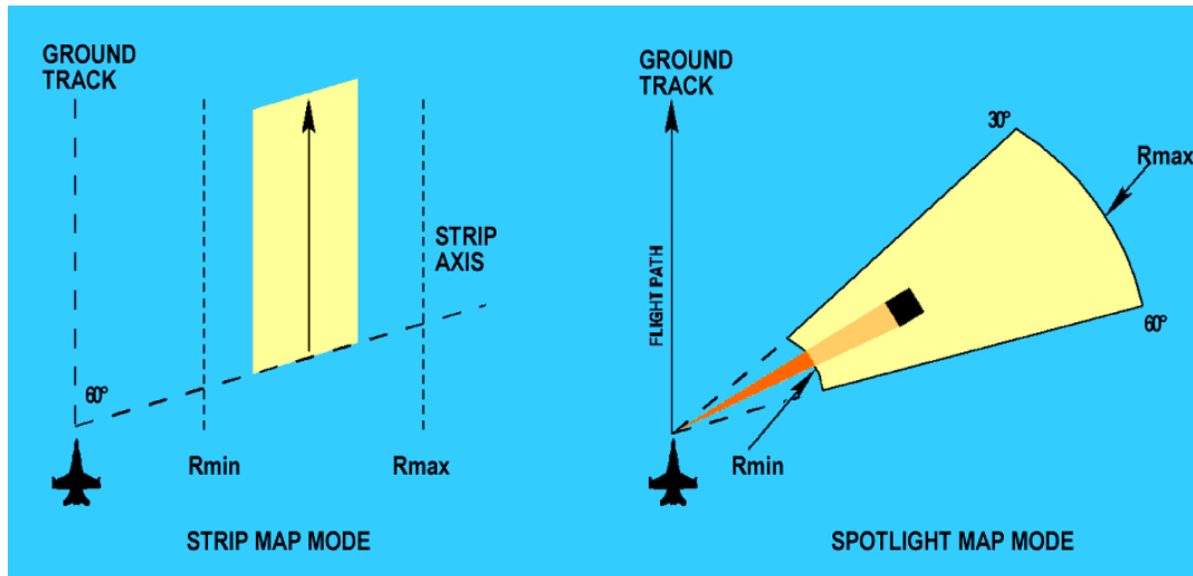
SAR Strip and Spot Light Modes Figure 4-3
