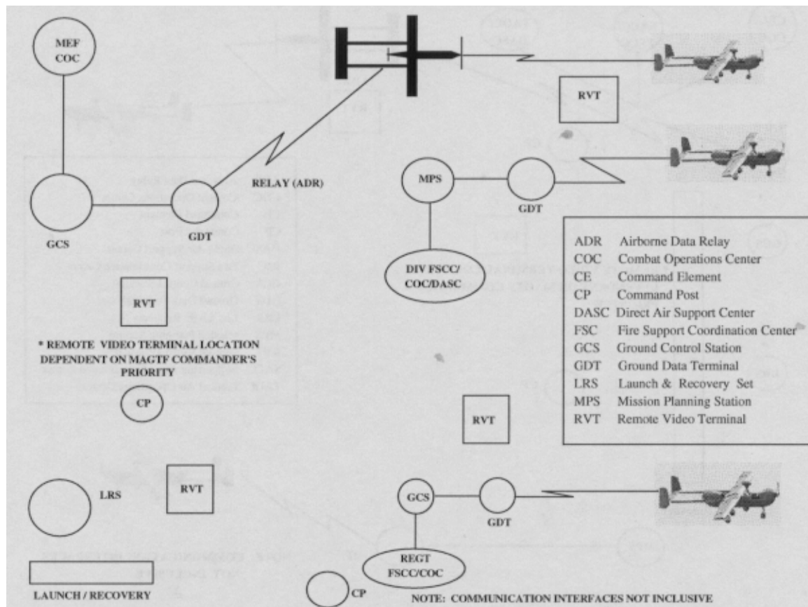
UAV System with Control Stations Figure 2-7
