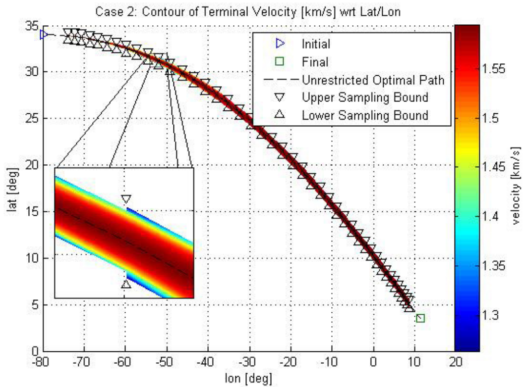
Figure 21. Case 2 contour of terminal velocity w.r.t. Lat/Lon.
