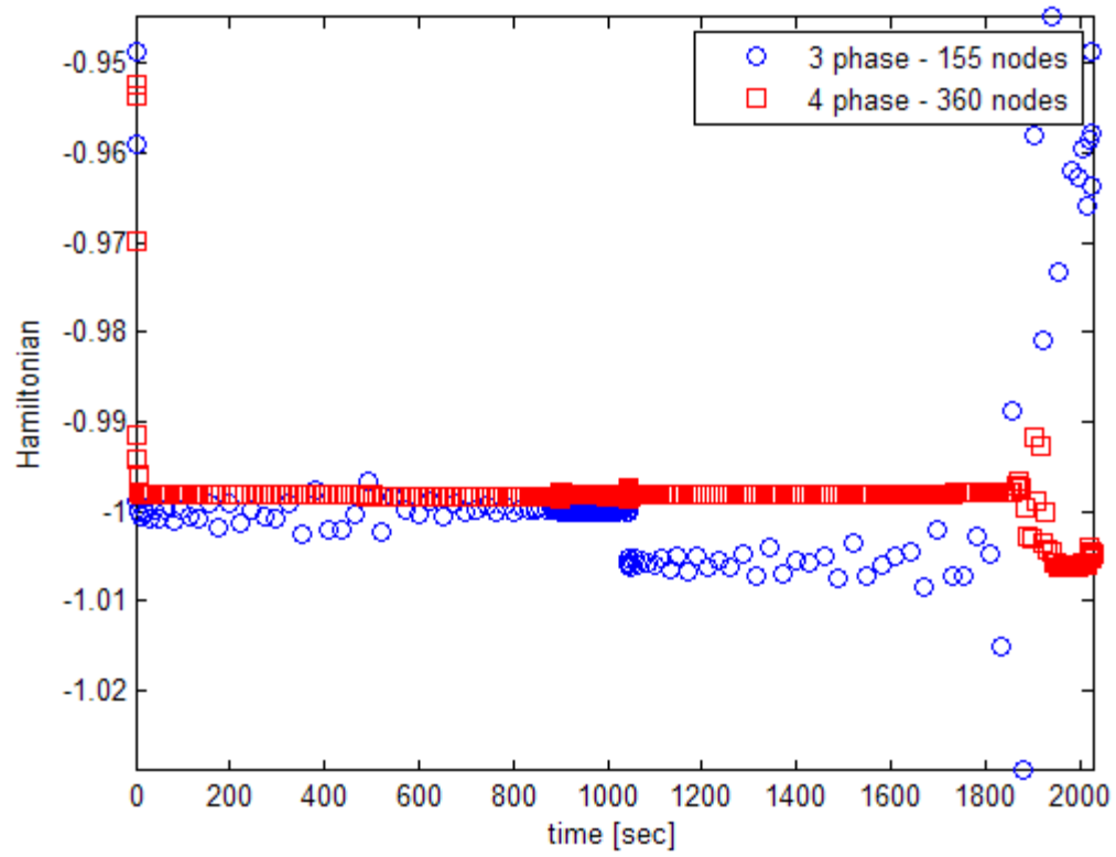
Figure 35. Hamiltonian of solution with 155 and 360 nodes.
