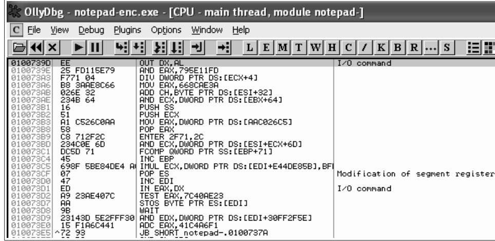
Figure 3.3: Runtime Disassembly of Protected Notepad.exe
