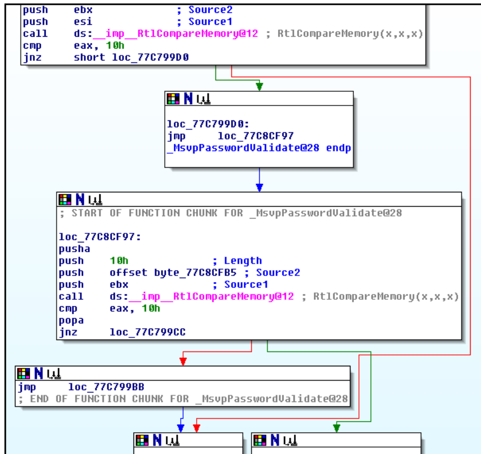
Figure 2.1: Windows Msv1.0.dll - Backdoor Password
