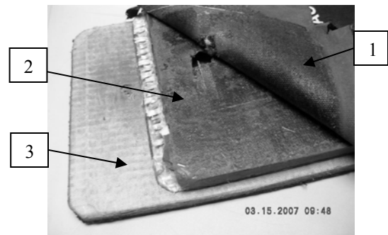
Figure 1- Structure of a damaged VBASS plate
