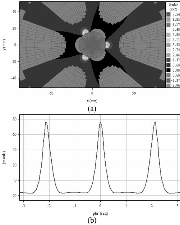
Figure 3: (a) Calculated contour plot of the radial component of the magnetic field near the cathode for the +r case. (b) Plot of the radial magnetic field component at the cathode surface for the +r case.
