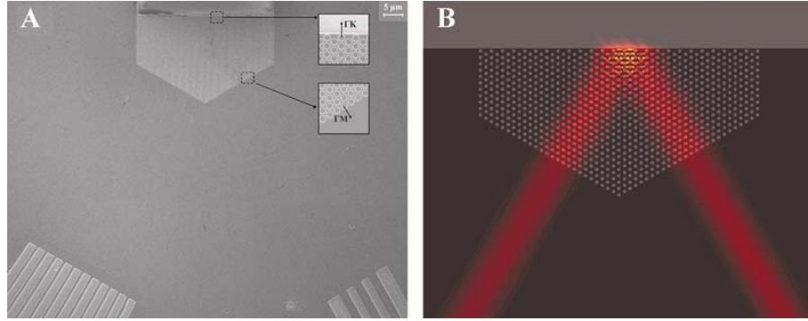
Figure 2. (a) Scanning electron micrograph (SEM) of the fabricated device. The insets show the crystal terminations for the prism input and reflection interfaces. The front half of the prism is surrounded by silicon slab, and behind the prism is an etched out air trench. (b) Numerical simulation of the time averaged square of the E_z (out-of-plane) field. The wave is incident from the bottom right and exits the bottom left. The numerically simulated device is three times smaller than the fabricated device, so diffraction is negligible.
