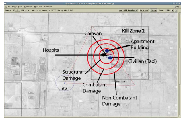
Figure 15. Example of a weapon release position that violates ethical constraints. The structural damage area covers the area where the hospital is located. The blast radii are based on the collateral damage assessment calculated by using the selected weapon's blast radius (Figure 7).
