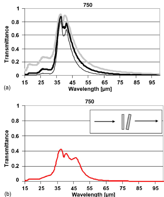
FIG. 12. (Color online) Transmittance of several 750 screens. (a) (Gray) One screen. (Bold black) Two screens. (Black) Three screens. (b) Two screens at an angle of 15^\circ .
