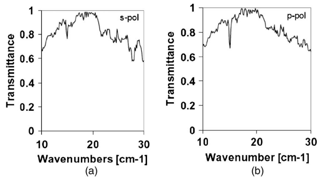
FIG. 9. Experiment with laser light: Transmittance of s - and p -polarized beams for screen 55 at normal incidence. (a) s polarization. (b) p polarization.
