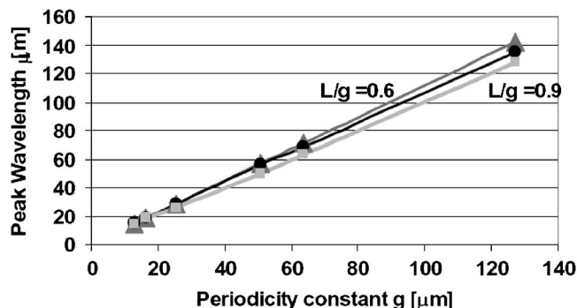
FIG. 14. Simulations: Peak resonance wavelength as a function of g and L . (Dark gray triangles) L/g=0.6 . (Black circles) L/g=0.75 . (Light gray squares) L/g=0.9 .
