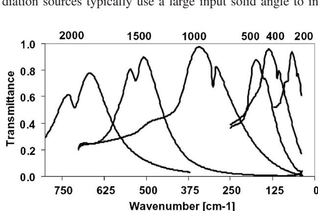
FIG. 1. Transmittances of nickel screens of 2000, 1500, 1000, 500, 400, and 200 lines/in. obtained with Bruker FIR spectrometer at diverging incident angle of 17^\circ .
