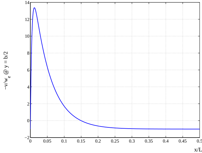
Figure 6: Meridional velocity in the middle of the basin adding no slip condition at the western boundary, i.e., v(x = 0) = 0 . \delta_s/L = 0.05 and \delta_{sub} = 0.0045
