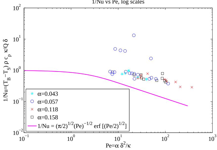
Figure 12: Variation of inverse Nusselt number 1/\text{Nu} = (T_B - T_S)\rho c_p \kappa / Q \delta with Péclet number \text{Pe} = \alpha \delta^2 / \kappa , plotted on logarithmic scales. The non-dimensional form of the Osborne (1965) prediction (23) is plotted with a solid line for comparison.
