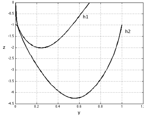
Figure 5: Plot of variation of the with latitude y of the density interfaces at z = -h_1 and z = -h_2 for w_e = \sin(\pi f/f_0) .
