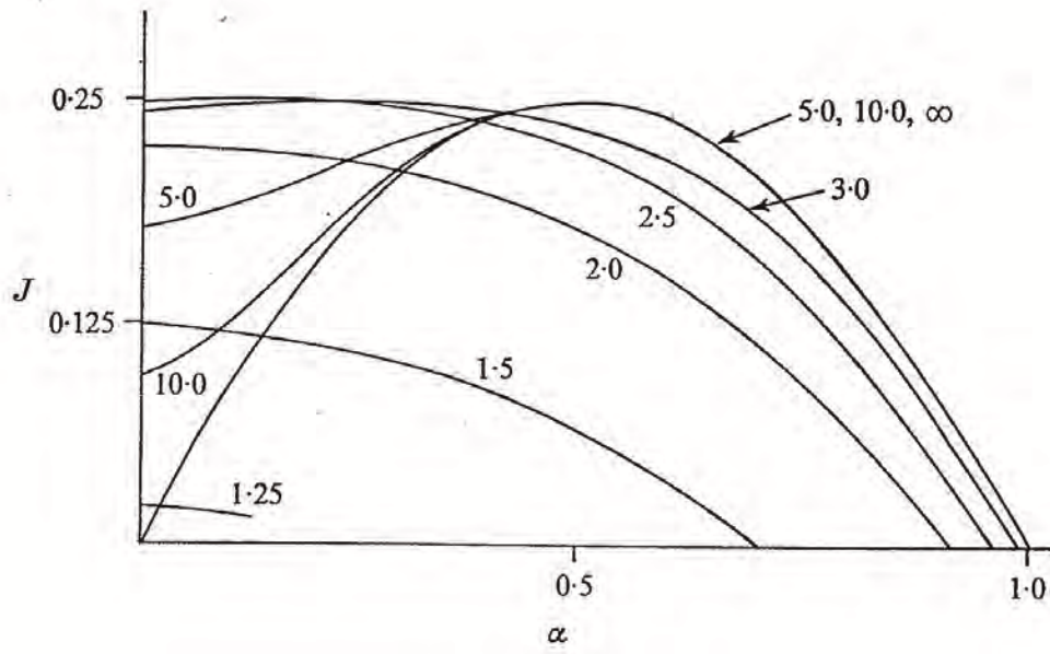
Figure 1: Stability boundaries for ‘tanh’ profiles at nondimensional distances marked. The vertical axis J represents the minimum Richardson number (found at z = 0 ) and the dimensionless wavenumber \alpha = kH for some typical length H . (Taken from Hazel (1972)).
