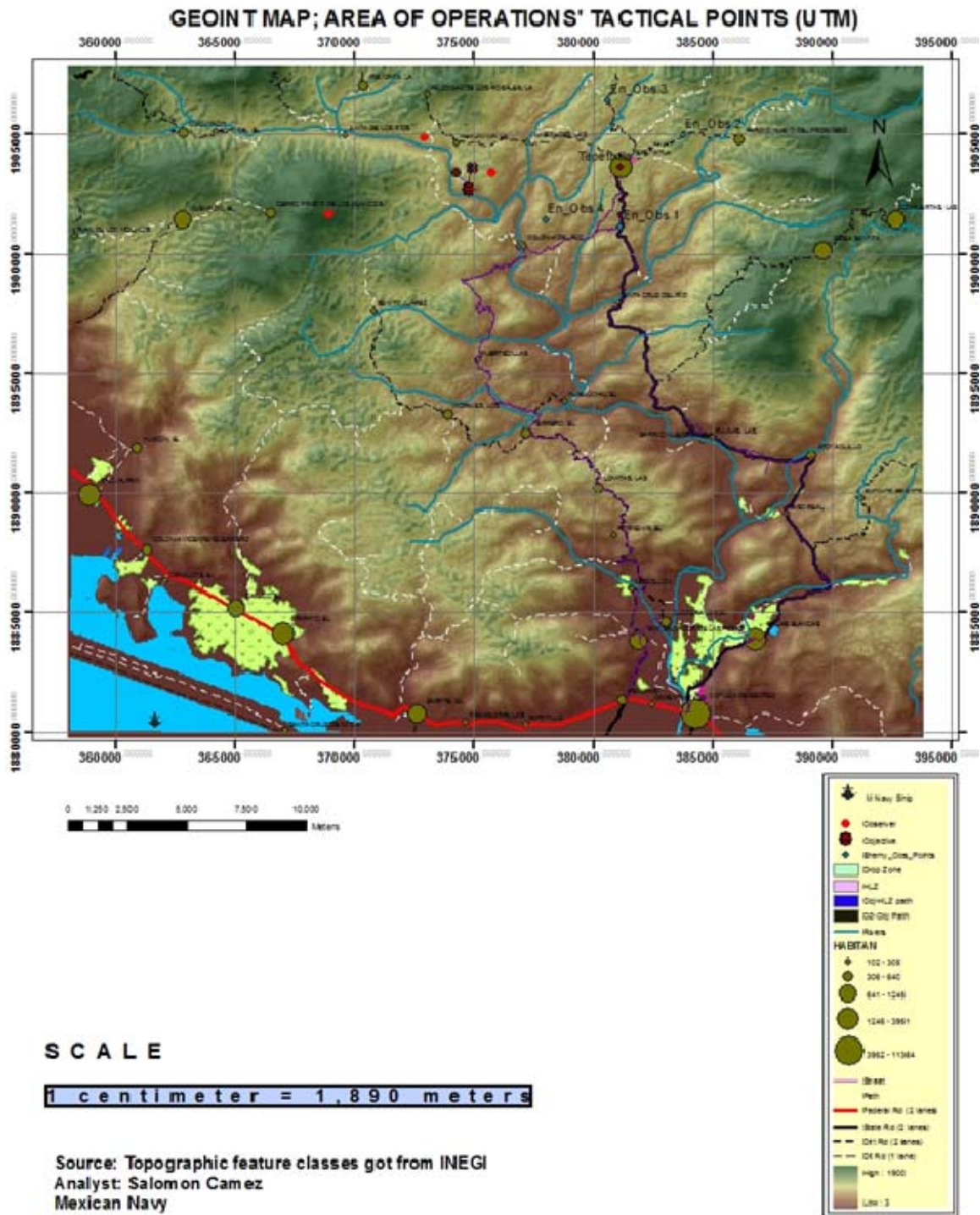
Figure 87. GEOINT Operational Map in UTM
