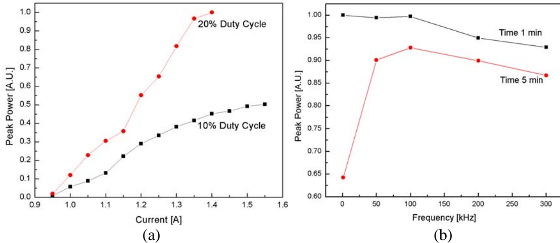
Figure 26. (a) Peak power of the device at 100 kHz for 10 and 20% duty cycles, with a pulse generator impedance of 50 \Omega into 13 \Omega at various currents, and (b) peak power of the device given a 10% duty cycle, with a pulse generator impedance of 50 \Omega into 13 \Omega at various frequencies after 1 and 5 minutes of lasing.
