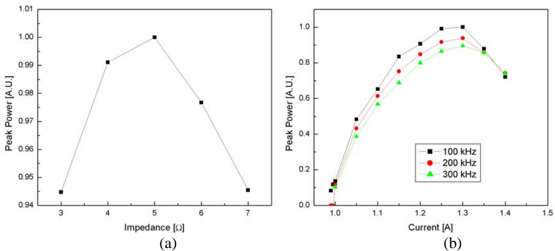
Figure 27. (a) 2.8 THz QCL peak power given a 10% duty cycle, and a pulse generator impedance of 50 \Omega into 3 to 7 \Omega , and (b) peak power given a 10% duty cycle, and a pulse generator impedance of 50 \Omega into 5 \Omega for various currents and PRFs.
