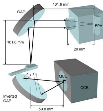
Figure 23. Schematics of the optics used in THz imaging.
