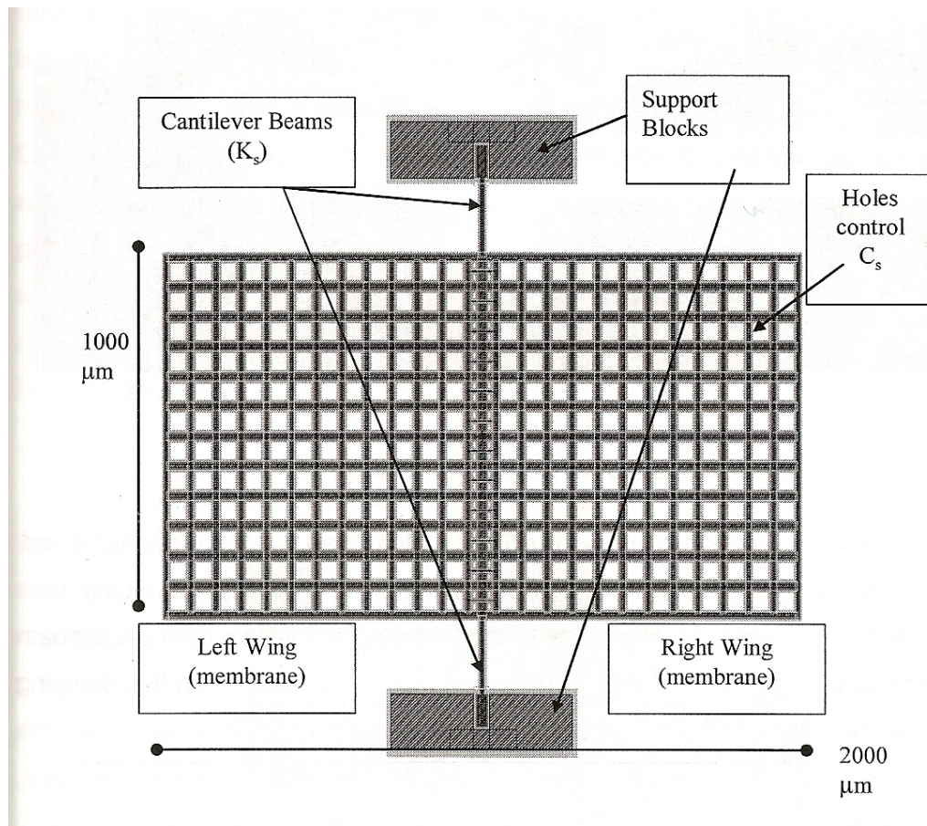
Figure 13. Initial design of a perforated MEMS device based on the PolyMUMPs' construction procedure (From: Shivok, 2007).
