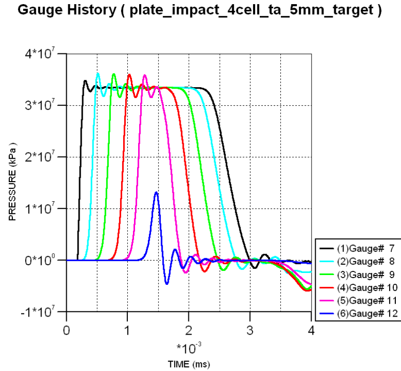
Figure 5. Pressure versus Time Plot of Plate Impact Simulation.
