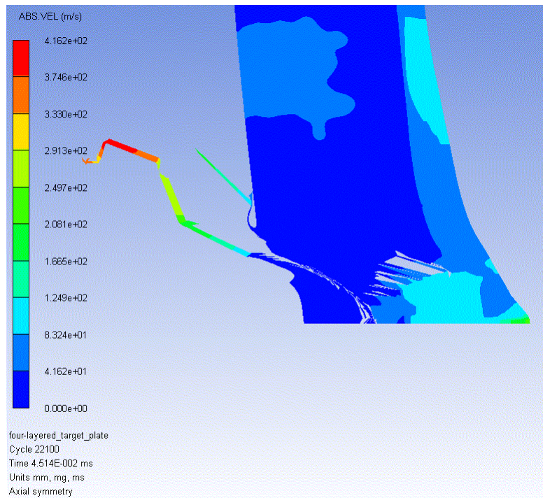
Figure 64. Velocity of Projectile of Layered Target Plate at 45μs.
