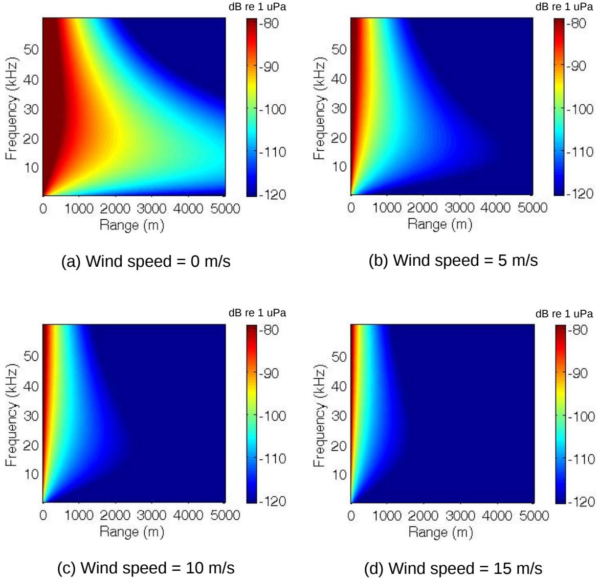
Figure 9. Effect of wind speed on -(TL + NL) in dB re 1\mu\text{Pa} . For a wind speed below 5 m/s, an acoustic communication range of up to 4 km is possible. As wind speed increases, communication range drops drastically.
