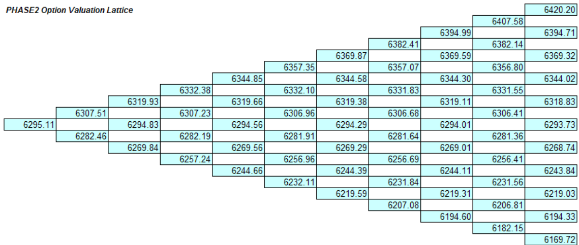
Figure 56. Phase 2 Option Valuation Lattice.
