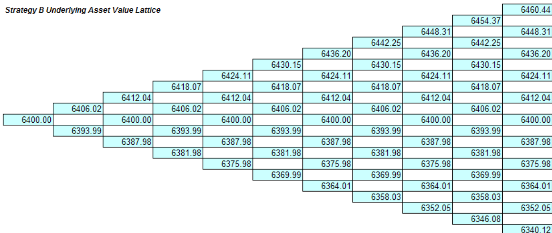
Figure 61. FCS Network Underlying Asset Lattice of with Deferment Option.
