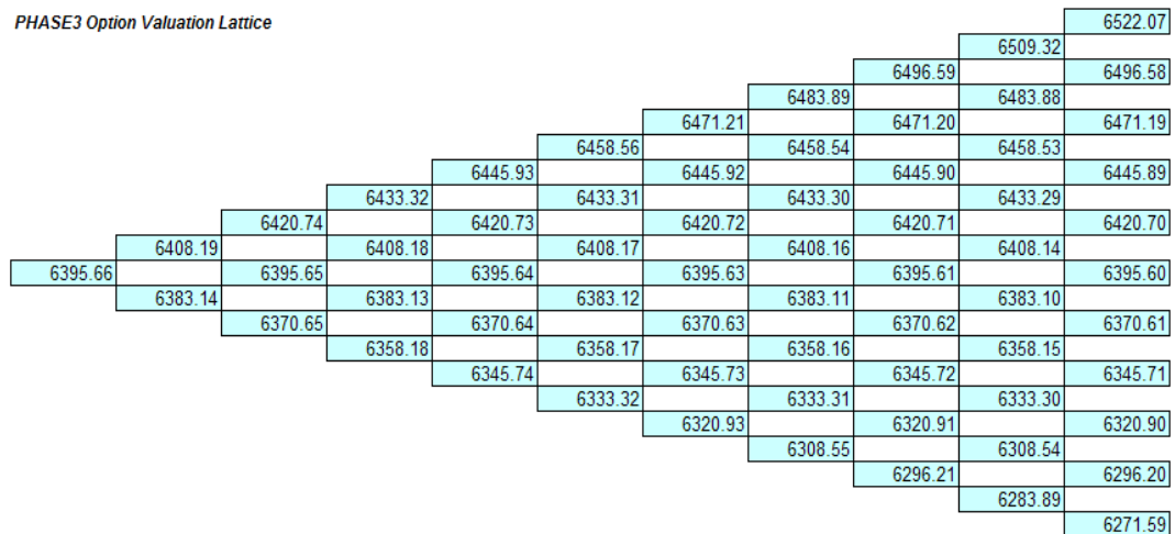
Figure 57. Phase 3 Option Valuation Lattice.
