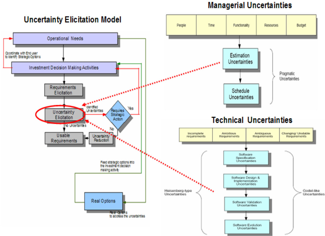
Figure 19. Expanded View of Uncertainty Elicitation Model.
