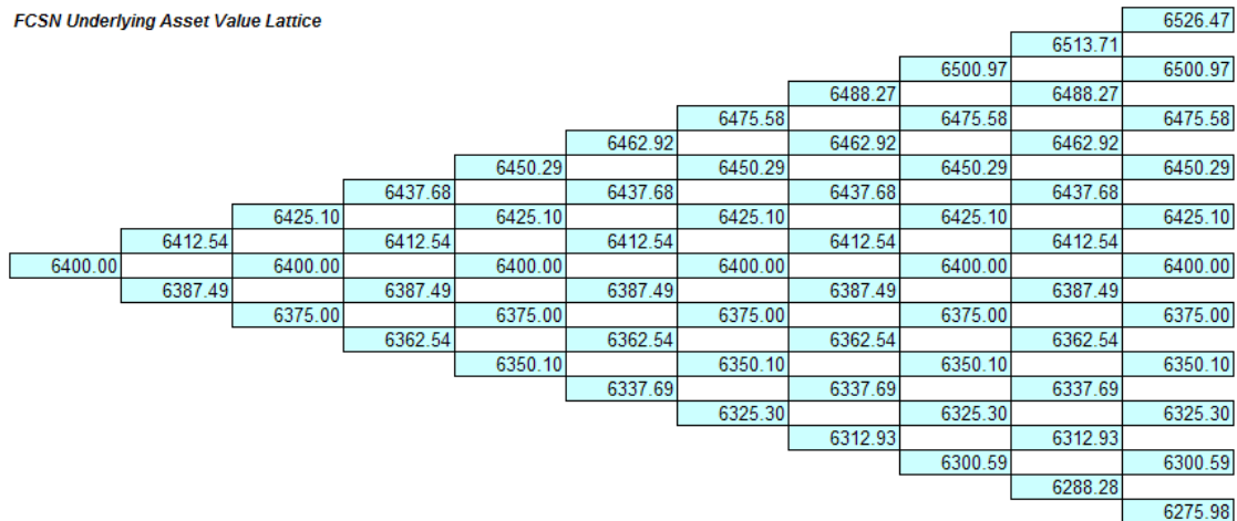
Figure 54. Lattice of Underlying Asset (FCS Network).
