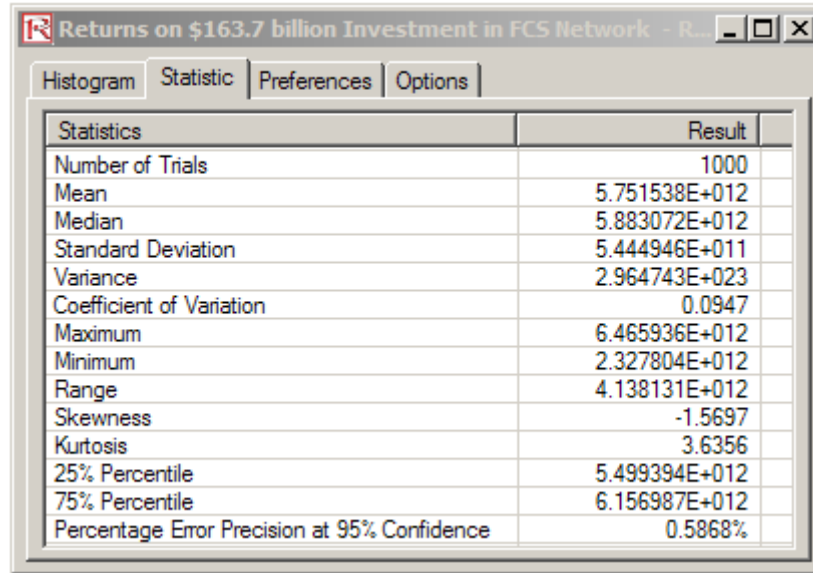
Figure 51. Revised volatility of the returns on the $163.7 billion Investment in the FCS Network. The forecast statistics summarizes the distribution of the forecast values in terms of the four moments of a distribution.
