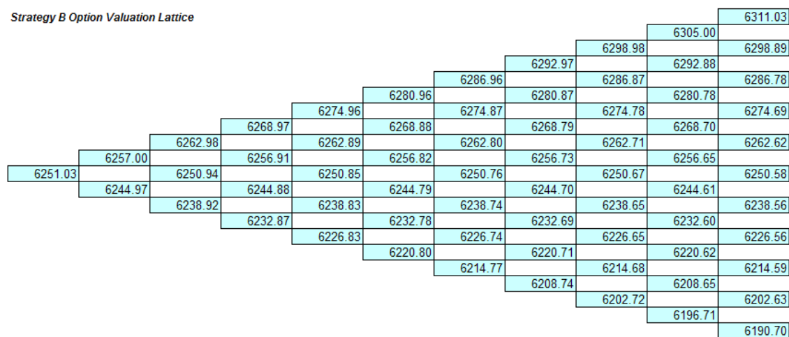
Figure 62. Options Valuation Lattice under Deferment.
