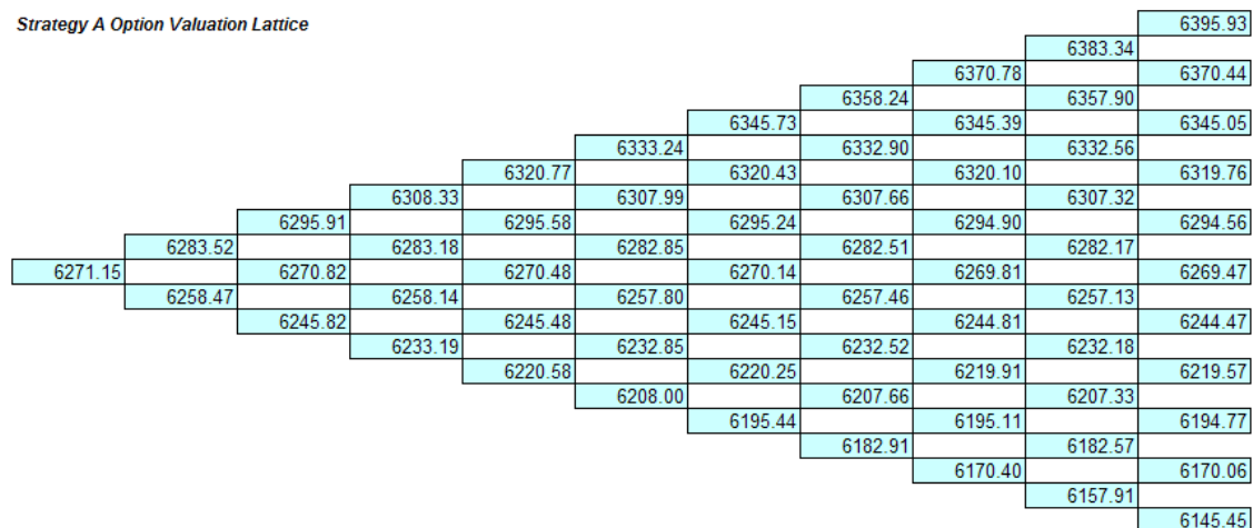
Figure 55. Phase 1 Option Valuation Lattice.
