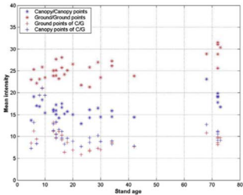
Figure 12. LIDAR intensity (From: Kalogirou, 2006)
