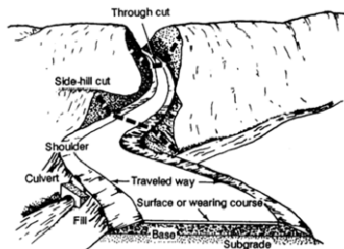
Figure 46. Road nomenclature
