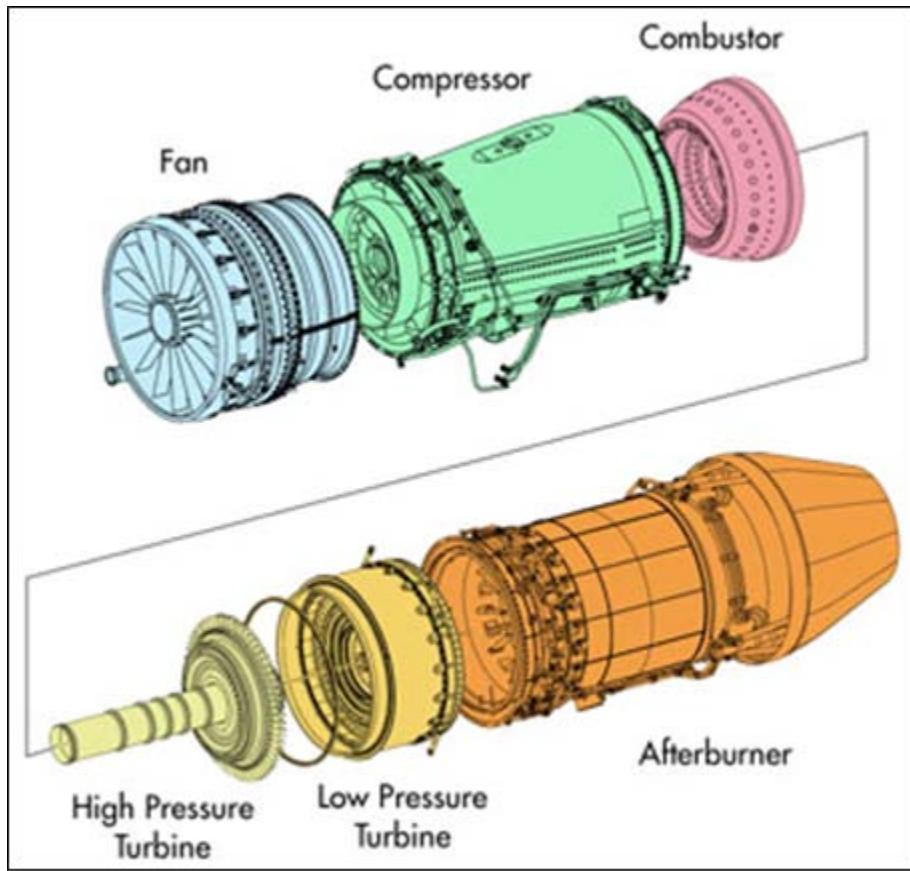
Figure 3. F414-GE-400 Engine Module Design (From: Defense Industry Daily, 2008)
