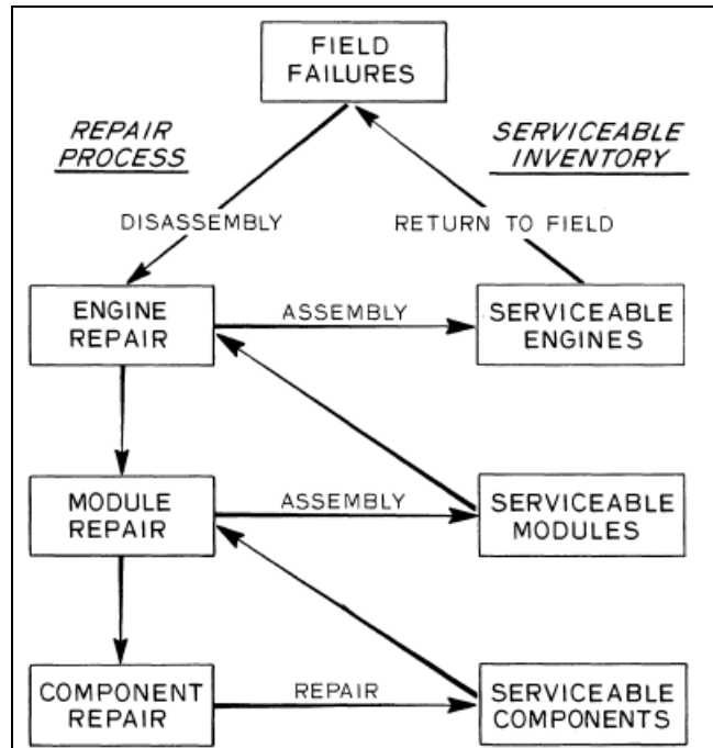
Figure 9. Remanufacturing Center Process Flow (From: Hausman & Scudder, 1982, p. 1,216)
