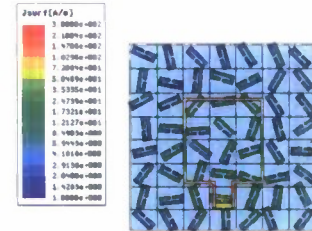
Fig. 6(e). Induced current on the random SRRs
