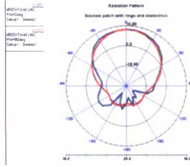
Fig. 18(b). Radiation pattern of the stacked patch with the SRRs
