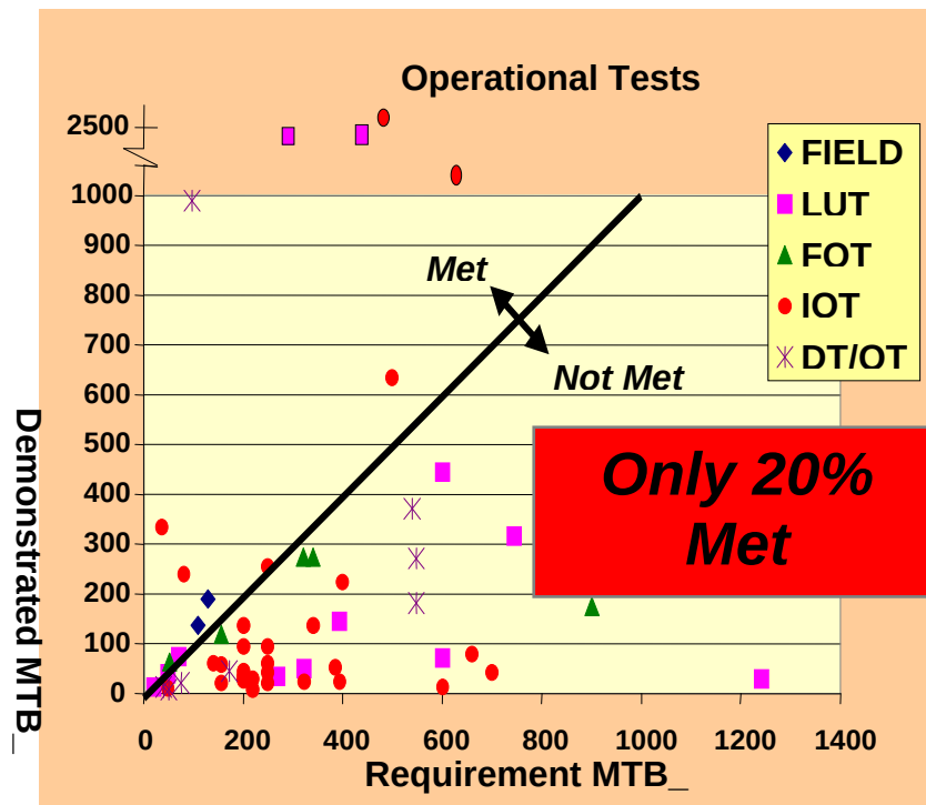
Figure 2. Reliability During Operational Tests (1996–2000) (Duma & Krieg, 2005)
