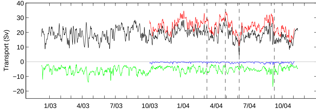
Figure 11. Absolute transports across the C-line. Red = positive, blue = negative onslope (countercurrent), green= negative offslope (recirculation), black = net. Tick marks denote the beginning of each month. Dashed lines show times of velocity snapshots plotted in Figure 8.
