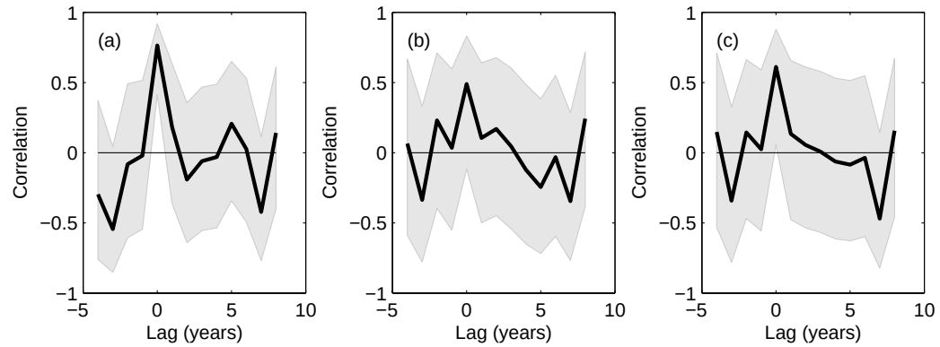
Figure 43. Lagged correlations of transports with PDO index.
