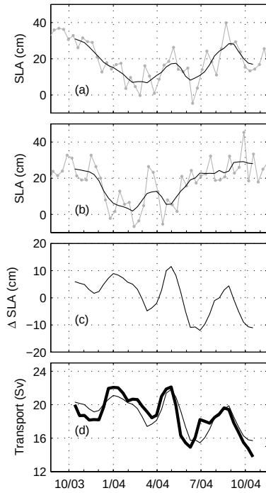
Figure 27. Satellite SLA timeseries.
