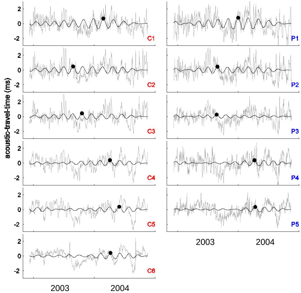
Figure 21. \tau records. CPIESs shown in left column and PIESs in right column. Two-day low-pass filtered records are shown in gray with 60 day (45-70) band-passed signals superimposed in black. For each record, the maximum in the band-passed record is highlighted with a filled circle (see text).
