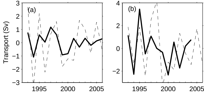
Figure 45. WBC transport anomalies.
