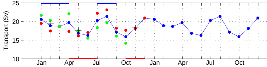
Figure 12. Monthly-mean net absolute transport. Red dots represent monthly means for the first year; green dots represent monthly means for the second year; blue dots represent monthly means for the two years averaged together (these are plotted and joined over a two year period to show clearly the yearly cycle). + = seasonal (3-month) means for the two years averaged together. Complete data for November and December are only available for the first year. Red and blue bands show periods of Kawabe's (1988) semiannual-type minima and maxima, respectively (see text).
