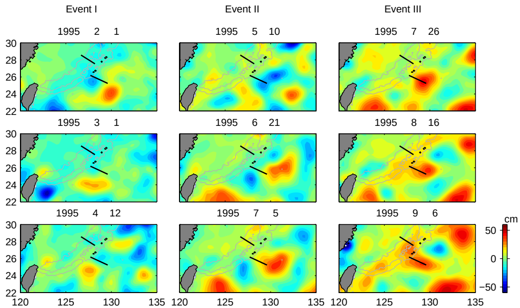
Figure 35. Merged satellite SLA maps.
