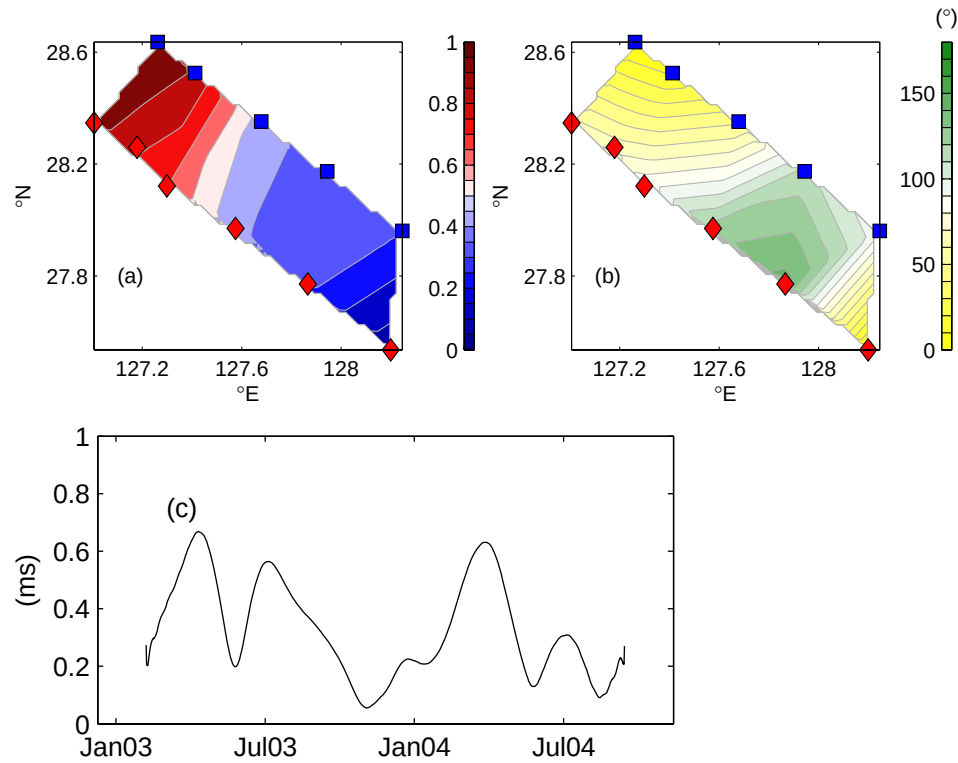
Figure 19. 1 st mode CEOF of 11-day (10-12) \tau . Panels show (a) magnitude, (b) phase, with propagation from high to low values, and (c) amplitude time series. Locations of CPIESs (red diamonds) and PIEs (blue squares) are shown. Tick marks denote beginnings of designated months.
