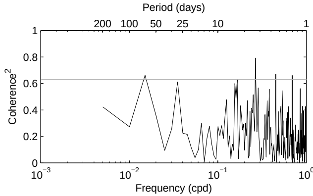
Figure 23. Coherence-squared between \tau at C1 and the area integrated wind stress curl. Area of integration is over the ECS shelf region 26°N - 33°N, 121°E - 125°E. Gray horizontal line shows the 95% confidence level (0.63).
