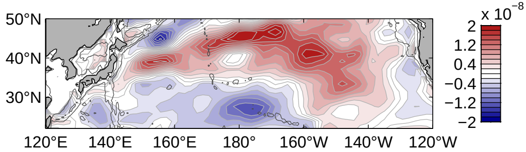
Figure 46. Annual mean \nabla_H \times \tau_w regressed onto annual mean PDO index anomalies. Contour interval is 0.2 \times 10^{-8} \text{ N/m}^3 . Isobaths are shown at 500 and 3000 m depth.
