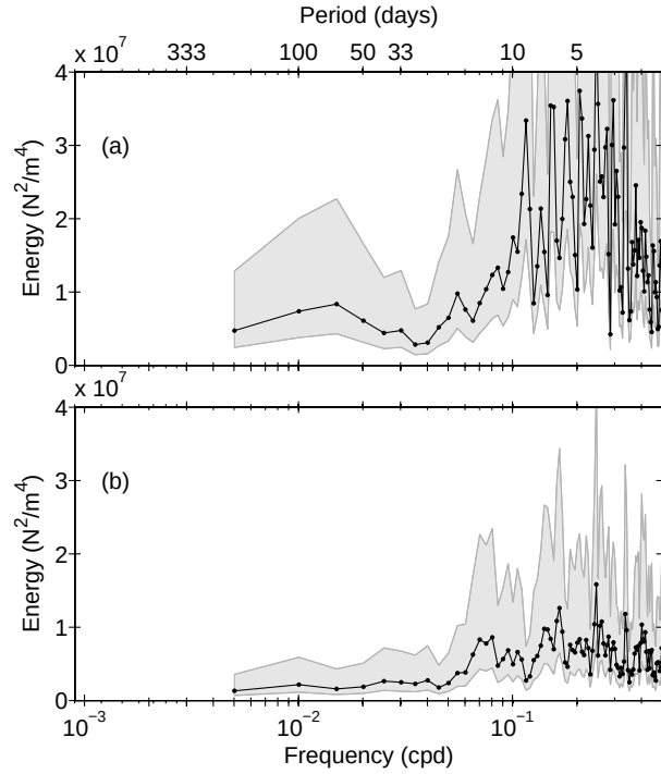
Figure 22. Variance preserving spectra of area-integrated wind stress. Panel (a) shows y wind stress and (b) shows x wind stress. Area of integration is over the ECS shelf region 26°N - 33°N, 121°E - 125°E. Analysis parameters are as in Figure 14.
