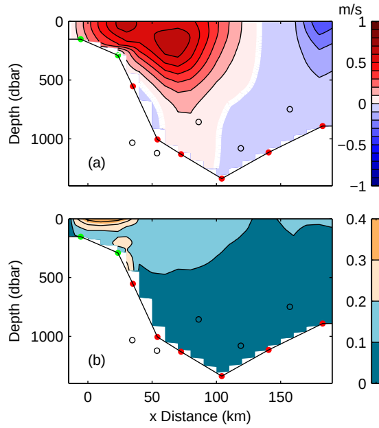
Figure 7. Velocity mean and standard deviation. Velocity ( y -component) mean (top) and standard deviation (bottom) cross sections on the C-line. Here x = 0 at the shelf break (depth = 170 m). Green and red dots indicate locations of ADCPs and CPIESs, respectively. Open circles indicate locations of PIESs 40 km downstream from the C-line. 0.1 m/s contour interval; zero contour white.
