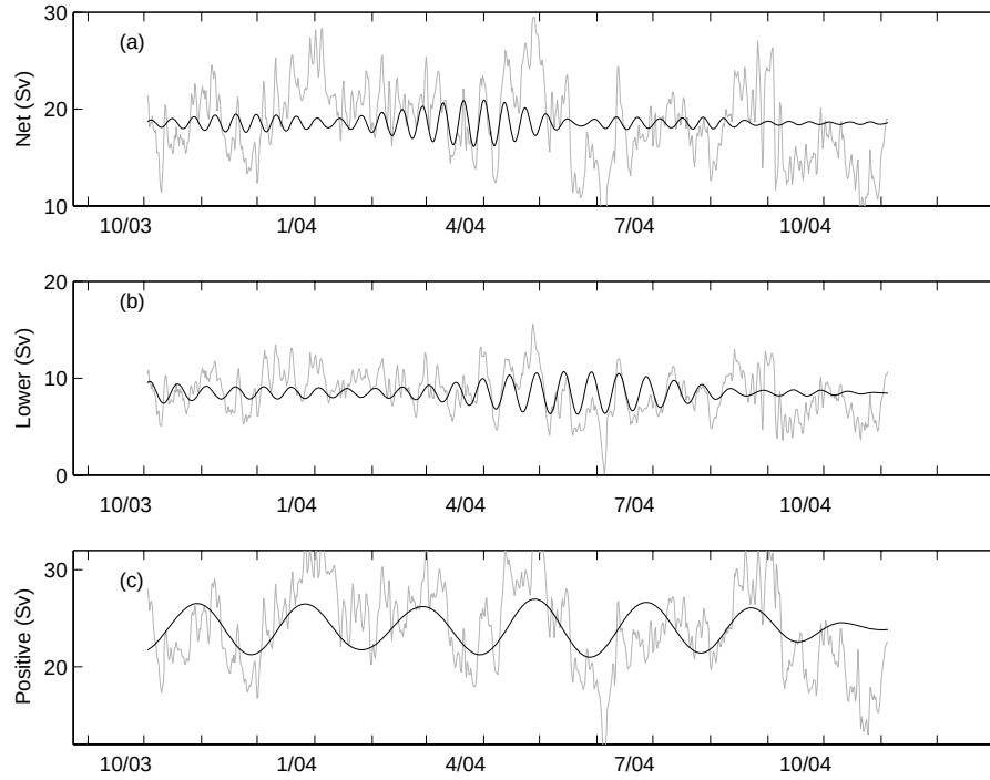
Figure 18. Band-passed transport time series. In all panels gray line is 2-day low-pass filtered transport and black line is band-passed signal. Panels show (a) net transport with 11-day band-pass (10-12), (b) lower layer transport with 15-day band-pass (13.5-16), and (c) positive transport with 60-day band-pass (45-70).
