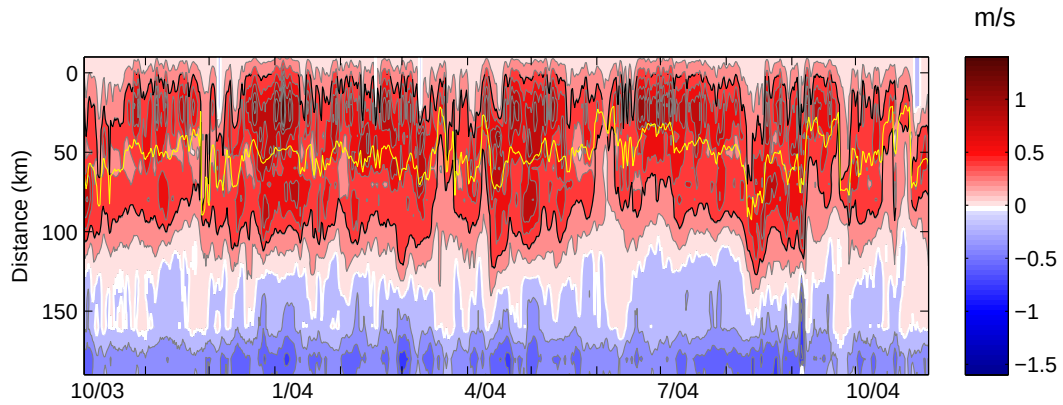
Figure 10. Surface velocity. Surface velocity (y-component) across the C-line shown on a t-x plot. Zero contour is white. Contour interval is 0.2 m/s. Black lines are edges of the Kuroshio “core” according to the definition of Guan (1980) and yellow line, mid-way between the black lines, is our “Kuroshio position.” Distances are given relative to the shelf-break (170 m depth). Tick marks indicate beginnings of months.
