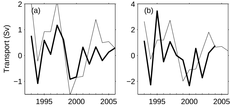
Figure 48. Comparisons of T_{Sv} and observed WBC transports. Panel (a) shows T_{Sv} calculated for the region between Taiwan and the Hawaiian Ridge (168.75°E) along 24°N with de-meaned ECS-Kuroshio transport shown for comparison (heavy solid line). Panel (b) as in (a) but calculated for the region between Okinawa and the Hawaiian Ridge (176.25°E) along 26°N with the heavy solid line showing the de-meaned Ryukyu Current transport.
