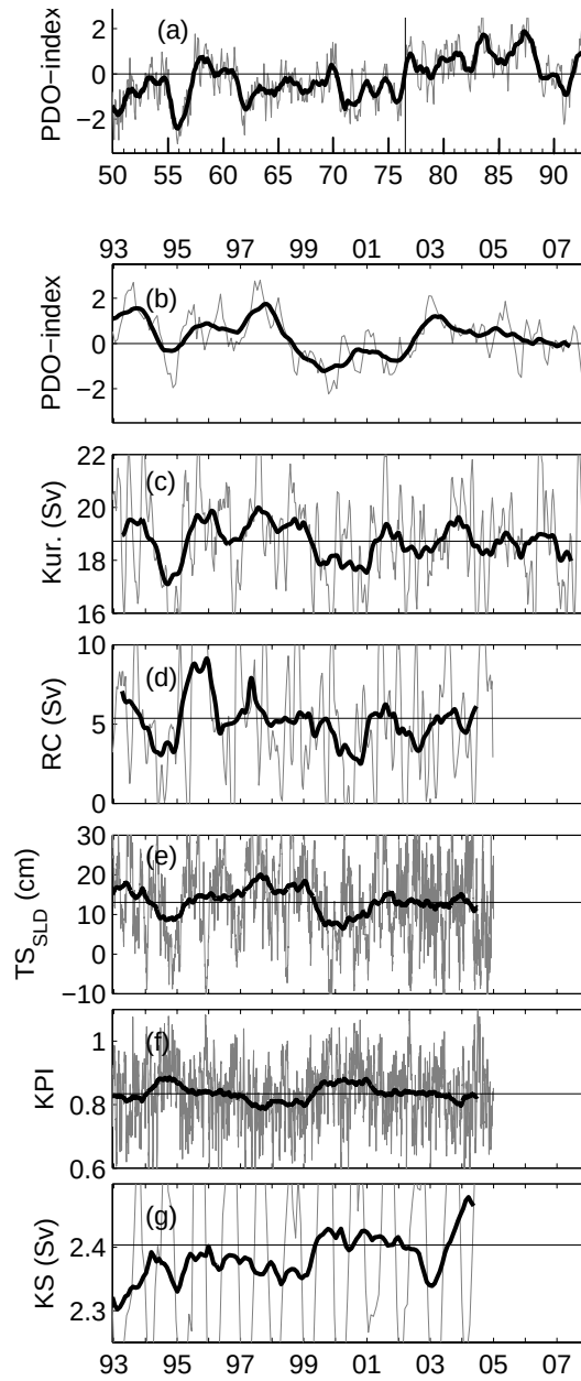
Figure 41. Time series comparisons with PDO index.
