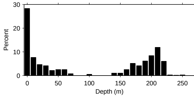
Figure 9. Histogram of depth of overall maximum velocity.
