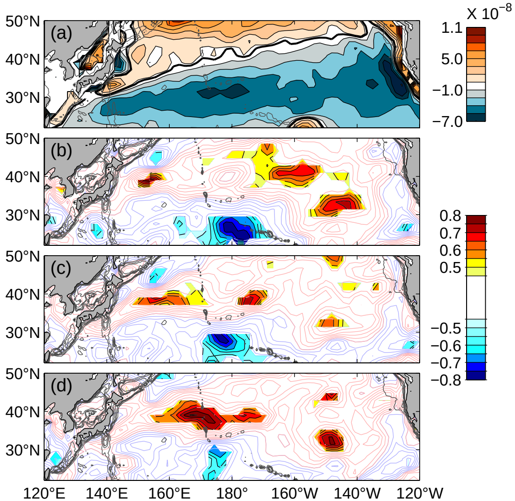
Figure 44. NCEP wind stress curl mean and correlation maps.
