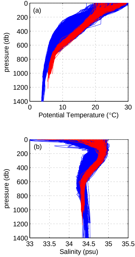
Figure 3. ECS hydrocast profiles. Panel (a) shows temperature and (b) shows salinity (b). Red are 113 profiles from Okinoerabushima Basin used to construct the localized GEM for C6. Blue are 1720 profiles from the rest of the ECS used to construct the main ECS GEM.
