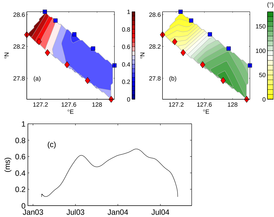
Figure 20. 1 st mode CEOF of 60-day (45-70) \tau . Panels show (a) magnitude, (b) phase, with propagation from high to low values, and (c) amplitude time series. Locations of CPIESs (red diamonds) and PIEs (blue squares) are shown. Tick marks indicate beginnings of designated months.
