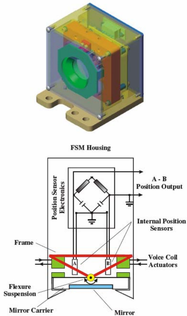
Figure 9 Typical FSM assembly showing the eight basic components
