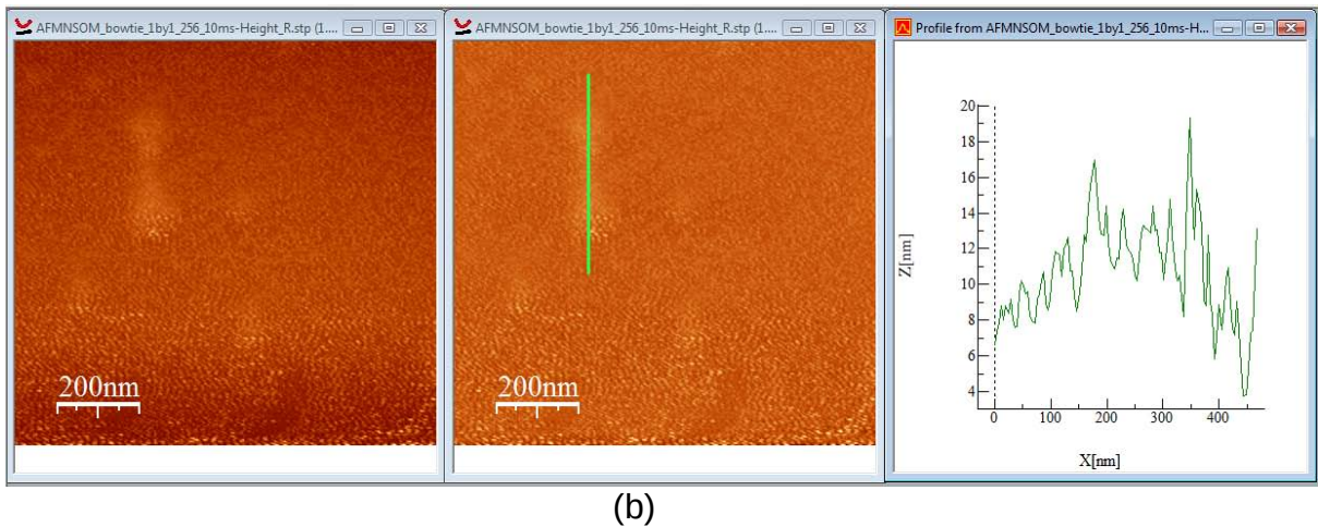
Figure 45 1μm by 1μm AFM Scan of a Pair of Nanobowties with (a) SEM Beam Off and (b) SEM Beam On.
