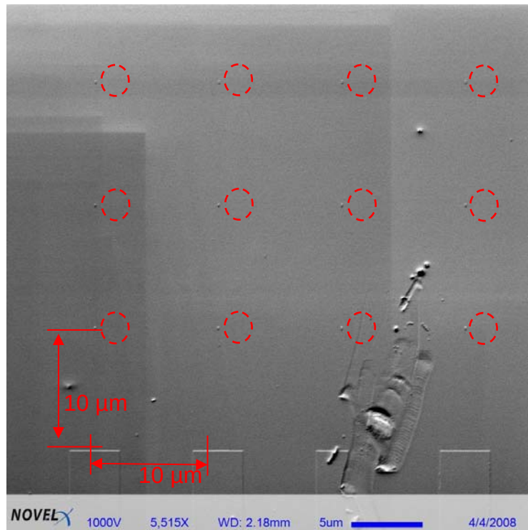
Figure 41 Au Nanobowties Array Fabricated on a GaAs Heterostructure with Au Strips of 10 μm Pitch to Demarcate the Locations of Nanobowties at 10 μm Intervals along Each Strip (Image Captured Using NovelX mySEM). This is the Actual Sample Used for this Thesis Work.
