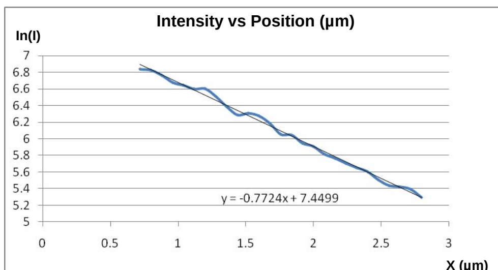
Figure 38 Semi-Log Plot of the Luminescence Intensity versus Distance for a 10 \mu\text{m} GaN Nanowire at its Narrow End ( \sim 100 nm).
