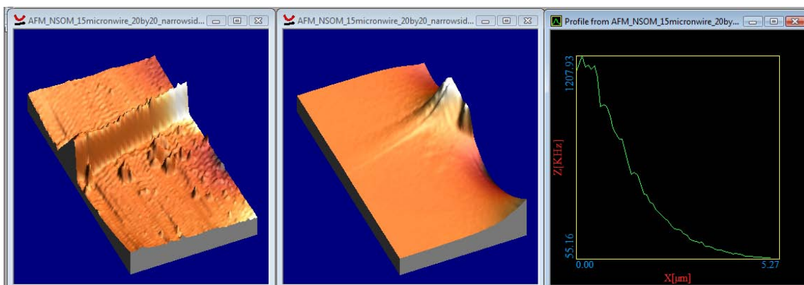
Figure 37 Profile of a 20-by-20 \mu\text{m} AFM/NSOM Scan of a 15 \mu\text{m} GaN Nanowire at its Narrow End ( \sim 100 nm).
