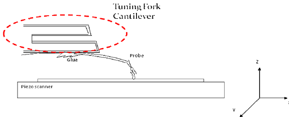
Figure 13 Schematic Diagram of the AFM/NSOM Probe.
