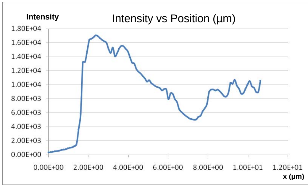
Figure 26 CL Intensity Map of GaN Nanowire in "Spot Mode" for \lambda = 660 nm.
