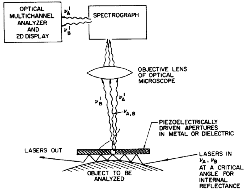
Figure 4 Schematic Diagram for Obtaining Spatial Resolution of 500 Å Using a Scanning Optical Microscope (from [15])
