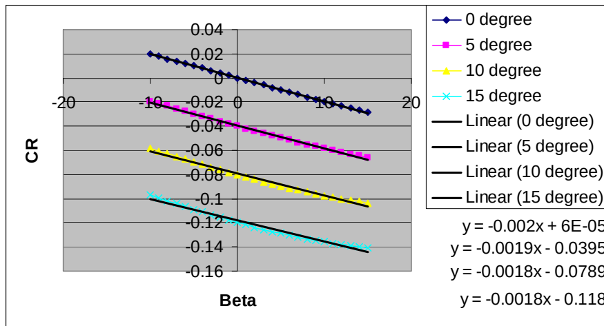
Figure 19. Curve for Cl_{Da}
