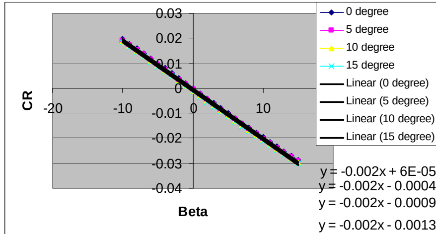
Figure 20. Curve for Cldr
