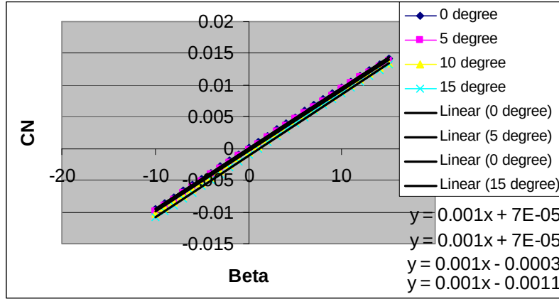
Figure 27. Curve for CN Da
