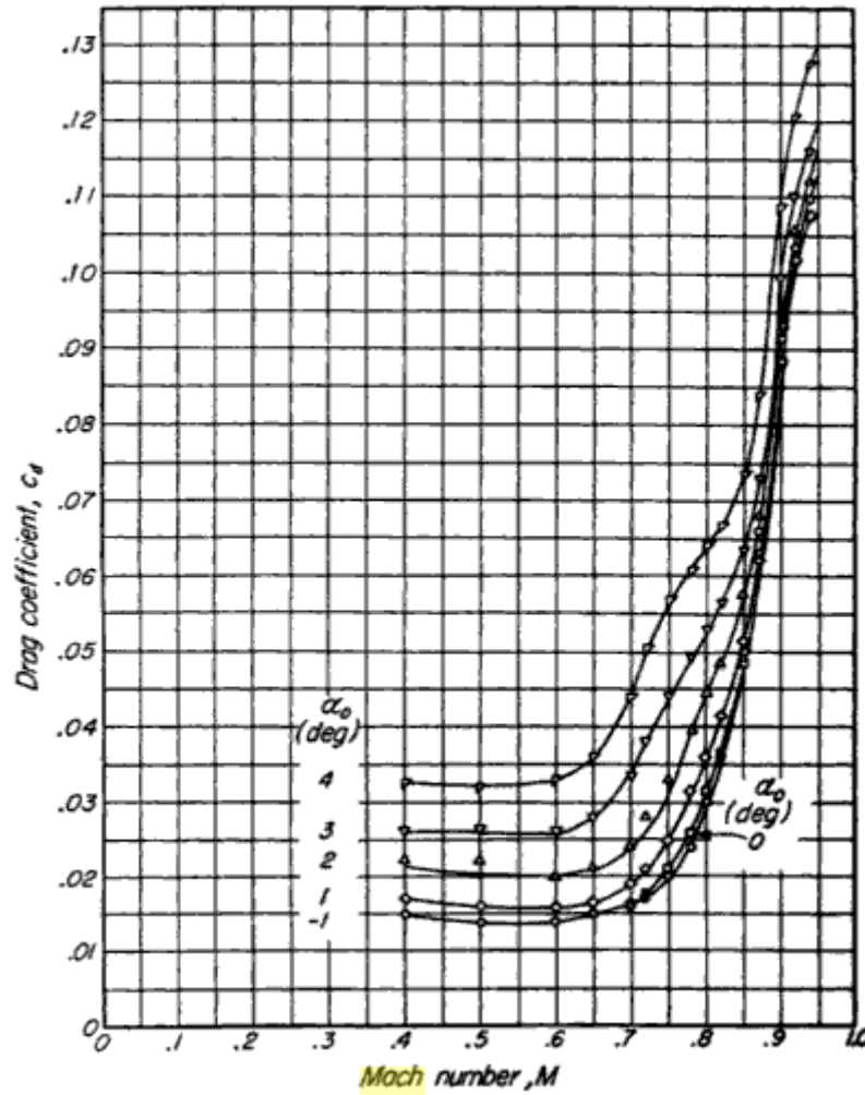
Figure 35. NACA 2312 Drag Coefficient vs. Mach [10]
