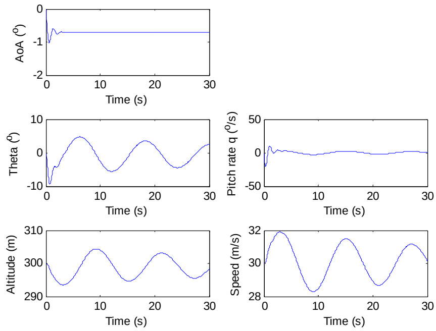
Figure 43. P10B longitudinal channel at trim condition
