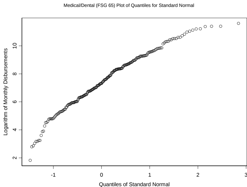
Figure 13. Plot of Standard Normal Quintiles for Logarithm of (1 + \text{Sum of Monthly Medical/Dental (FSG 65) Disbursements}) . From the 01 July 2007 to 30 April 2008 Dataset.
