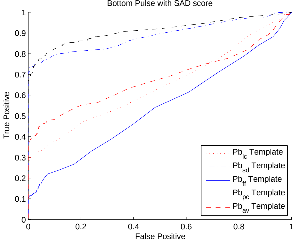
Figure 22. ROC graph of bottom-pulse templates with SAD
