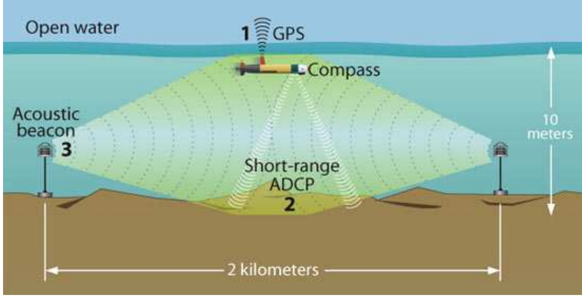
Figure 3. Different sensors REMUS uses for navigation in shallow water [Ref. 4].
