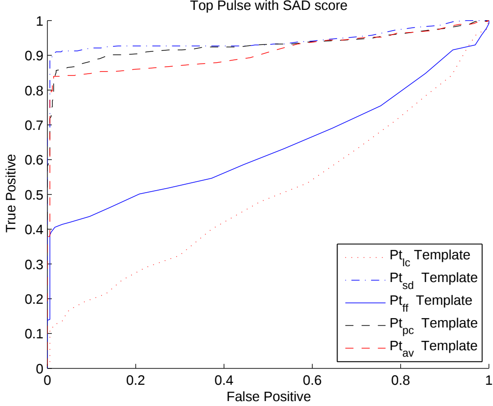
Figure 20. ROC graph of top-pulse templates with SAD
