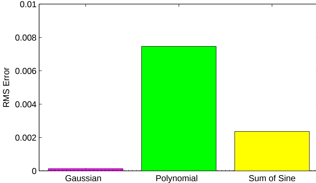
Figure 15. Graph of average RMS error of 1024 histograms for each of the three functions.
