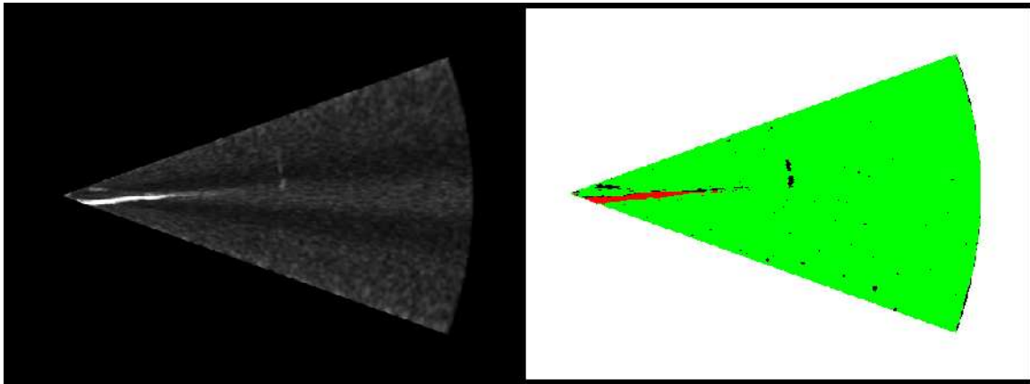
Figure 32. Left: Sonar Image with faint obstacle approaching. Right: Processed Sonar. Green=background, Red=ground, Black=unknown object
