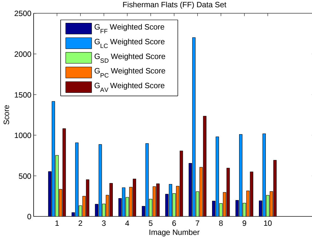
Figure 27. Plot of weighted score of five template fit to Fisherman Flats dataset
