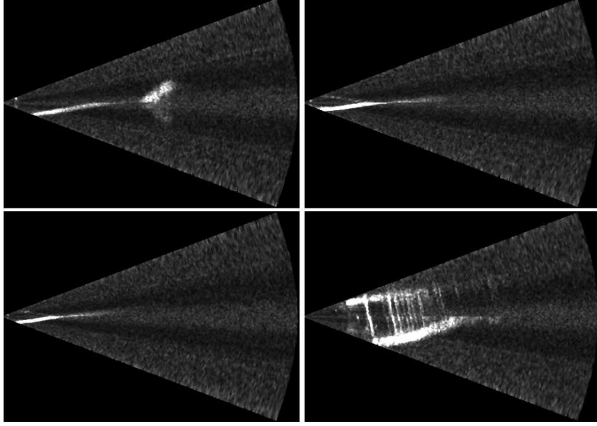
Figure 12. Sample Images from the four sites. Top Left: Fisherman Flats (FF) Top Right: Panama City (PC) Bottom Left: San Diego (SD) Bottom Right: Lovers Cover (LC).
