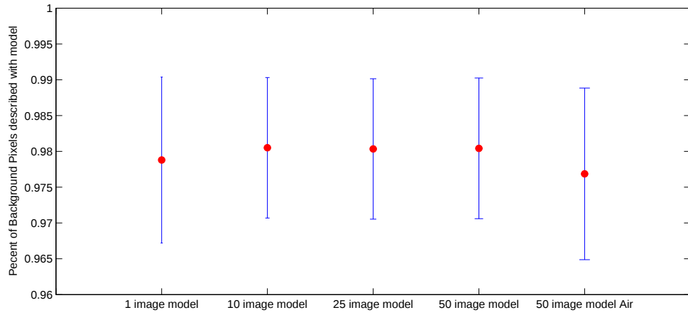
Figure 17. Percentage of pixels that fit within five different background intensity models.
