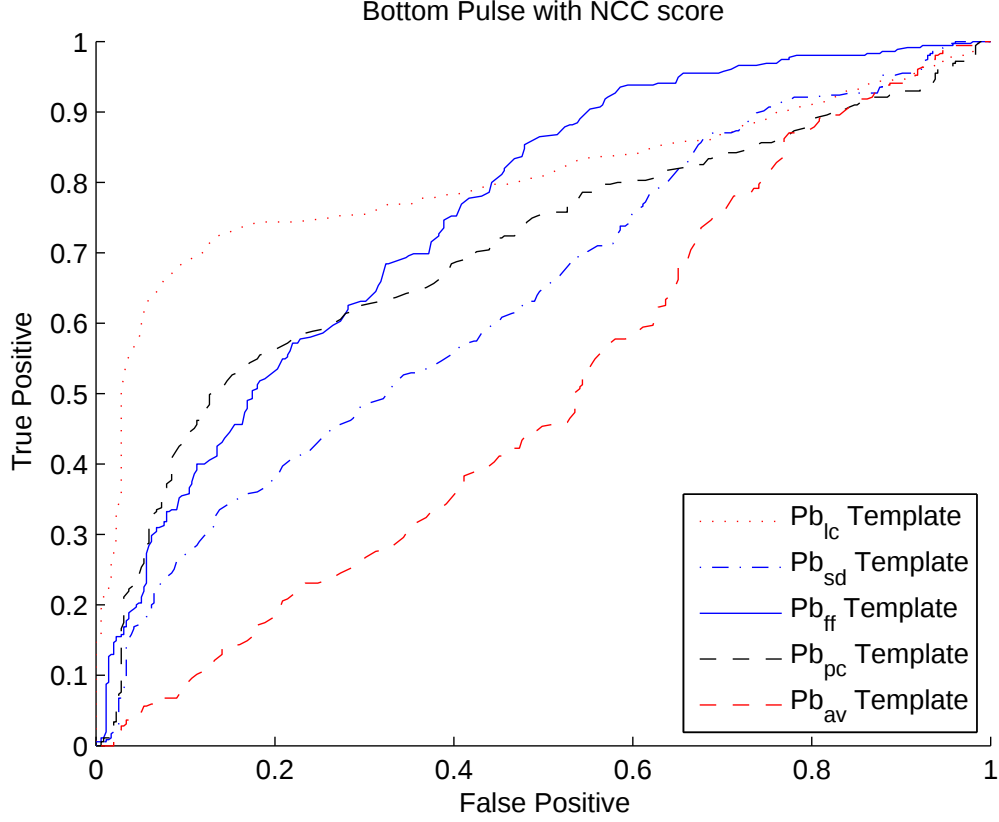
Figure 21. ROC graph of bottom-pulse templates with NCC
