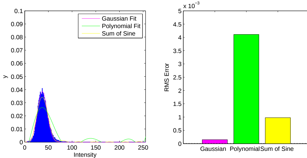
Figure 16. Left: Each of the 3 functions fit to the histogram. Right: Graph of the RMS error of each of the fittings.
