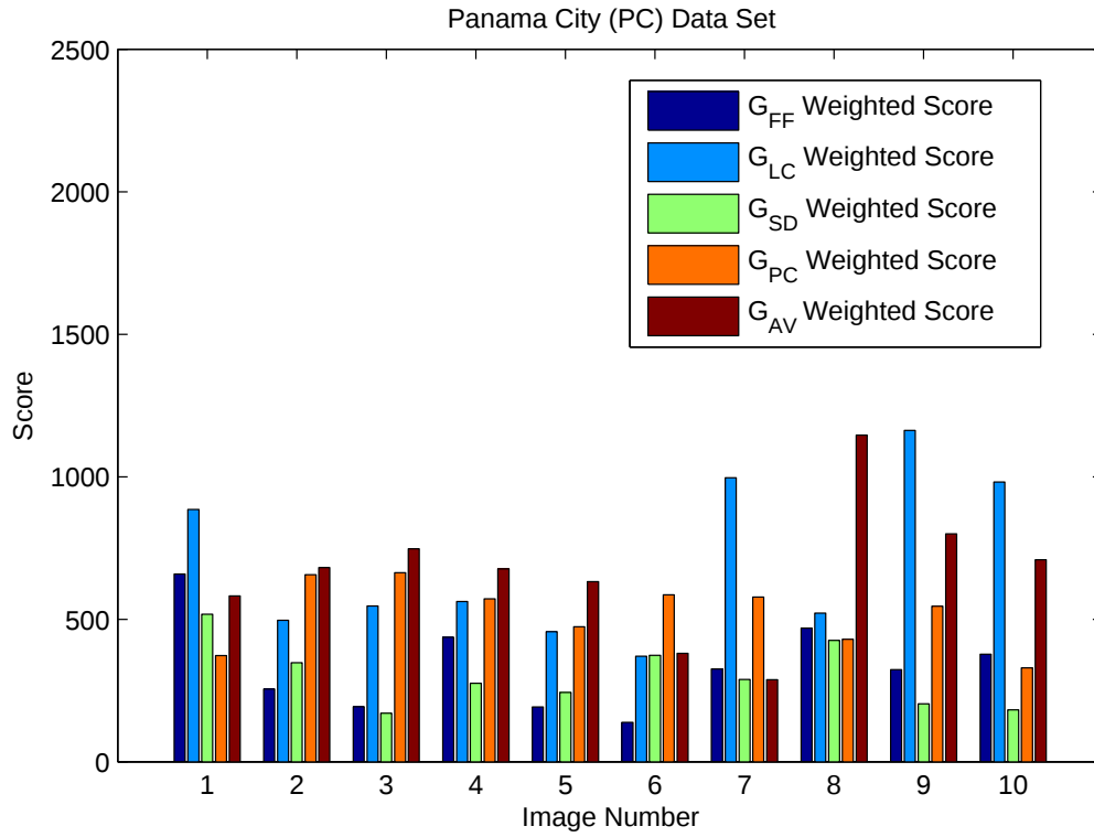
Figure 30. Plot of weighted score of five template fit to Panama City dataset
