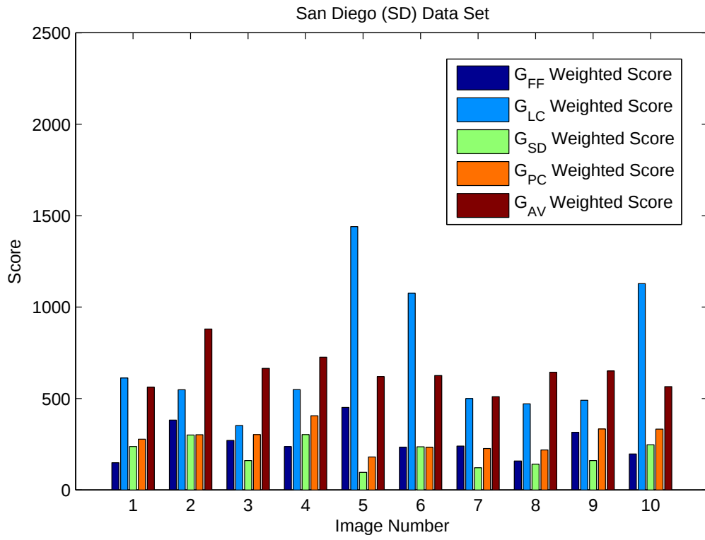
Figure 29. Plot of weighted score of five template fit to San Diego dataset
