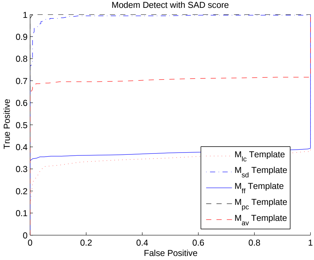
Figure 25. ROC graph of modem templates with SAD
