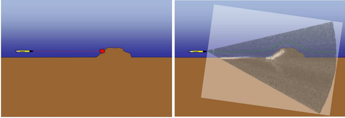
Figure 1. Left: Course with AUV flying above the ground on collision course with rock obstacle. Right: Actual forward looking sonar image overlaid on the schematic scene.
