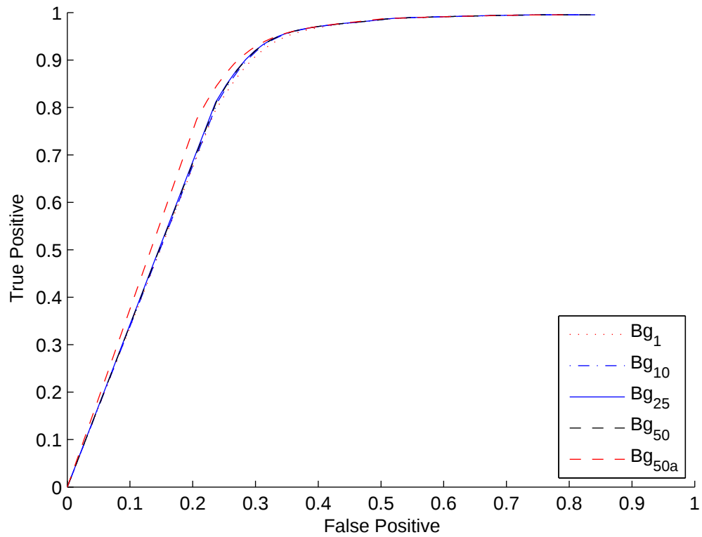
Figure 18. ROC curve of background classification.
