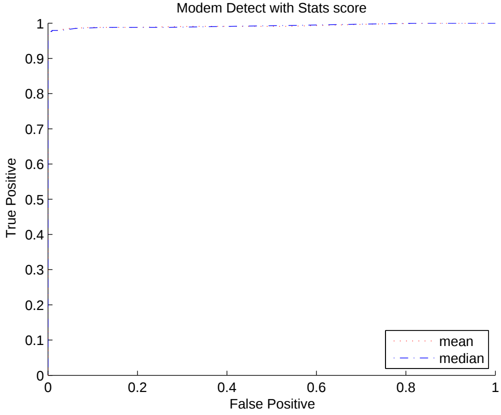
Figure 26. ROC graph of modem detection with statistic scores
