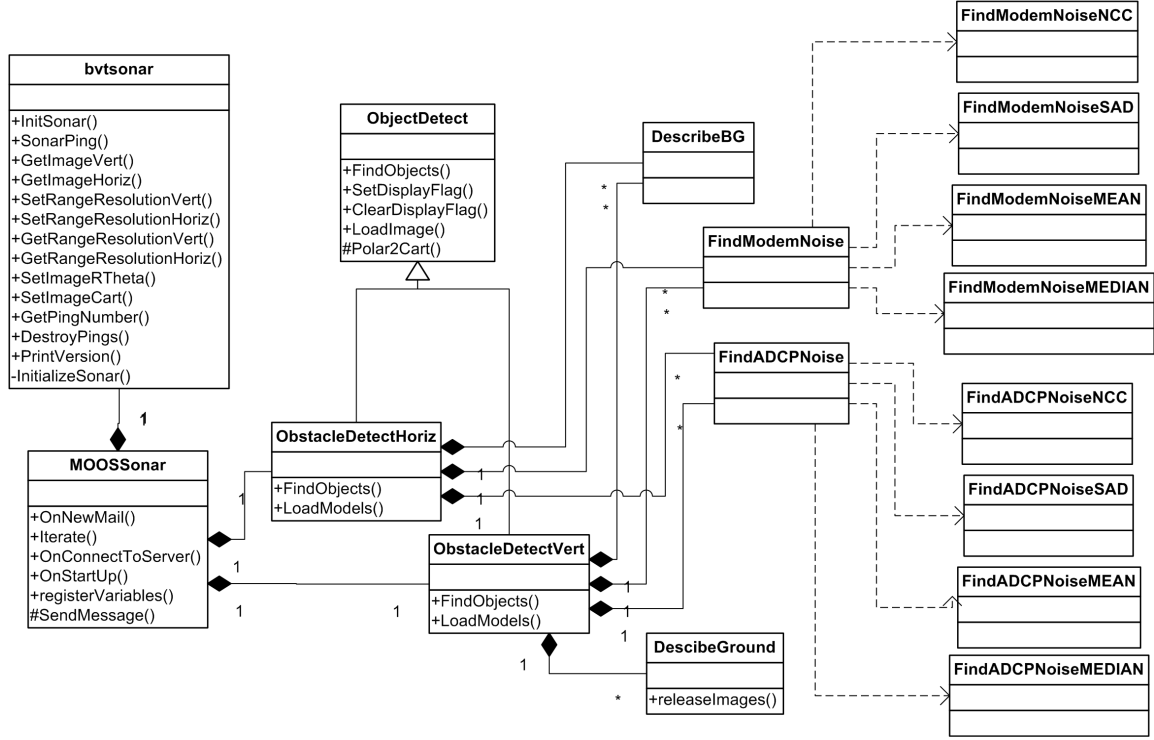
Figure 6. MOOS Module Class Diagram. This UML diagram was created after techniques were finalized in MATLAB. It served as a plan when developing C++ code.
