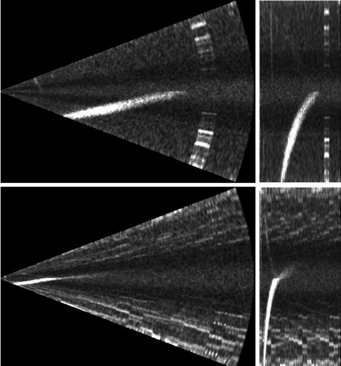
Figure 7. Top Left: Pulse artifact from unknown source and ground in Cartesian space. Top Right: Same image in Polar Space. Bottom Left: Modem noise and ground in Cartesian space. Bottom Right: Same image in Polar Space.
