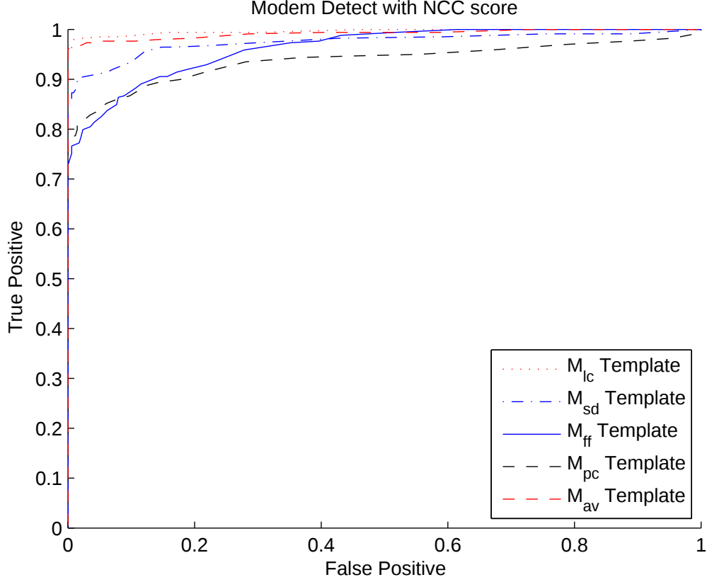
Figure 24. ROC graph of modem templates with NCC
