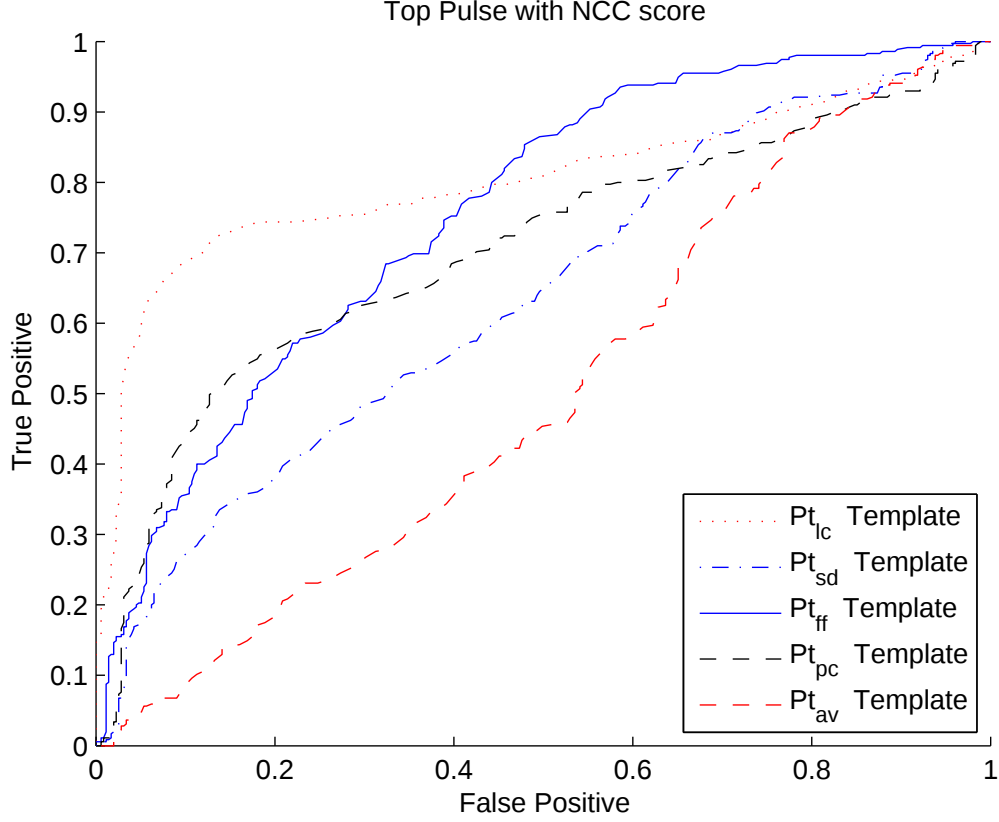
Figure 19. ROC graph of top-pulse templates with NCC
