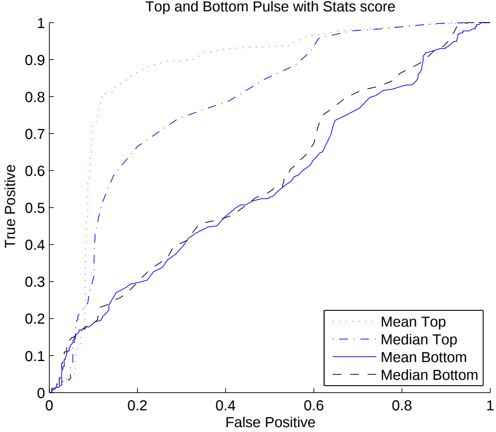
Figure 23. ROC graph of pulse templates with statistic test
