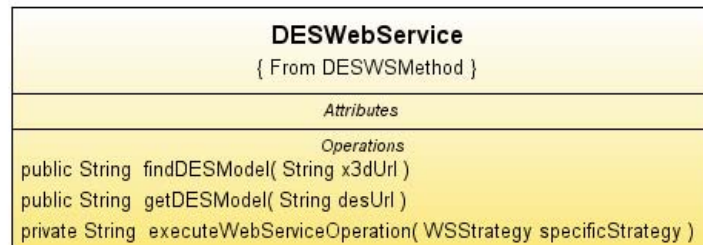
Figure 29. SAVAGE web services classes implemented in X3DWSMethod and DESWSMethod components. Class diagram in UML.
