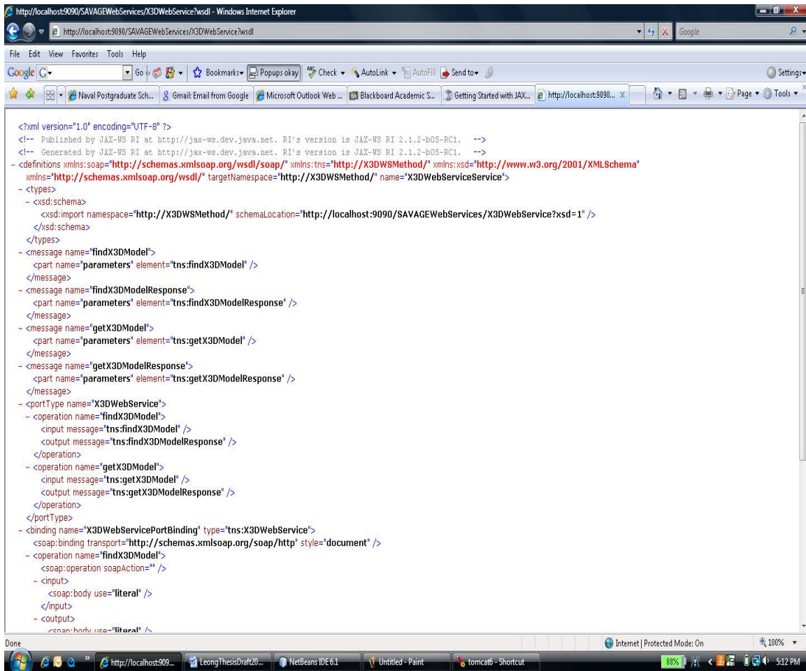
Figure 45. WSDL file that describes X3DWebService.
