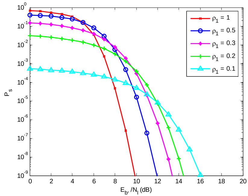
Figure 46. Probability of symbol error of a JTIDS/Link-16-type waveform for the single-pulse structure in both AWGN and PNI transmitted over a slow, flat Nakagami fading channel where m = 5 and E_b/N_0 = 15 dB.
