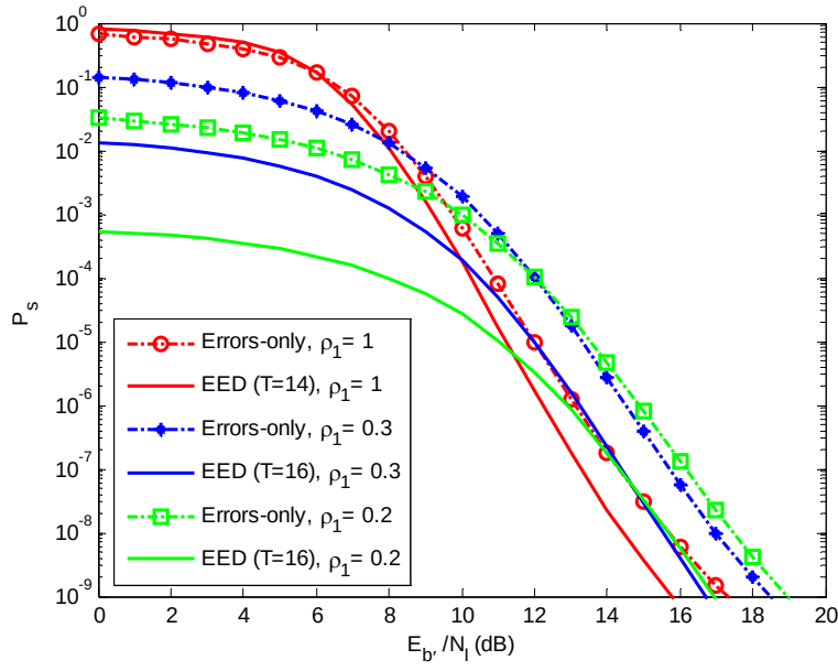
Figure 74. Probability of symbol error of a JTIDS/Link-16-type waveform for the single-pulse structure in both AWGN and PNI when the signal is transmitted over a slow, flat Nakagami fading channel where m = 2 and E_b/N_0 = 10 dB: EED versus errors-only RS decoding.
