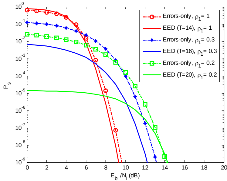
Figure 73. Probability of symbol error of a JTIDS/Link-16-type waveform for the single-pulse structure in both AWGN and PNI when the signal is transmitted over a slow, flat Nakagami fading channel where m = 5 and E_b/N_0 = 15 dB: EED versus errors-only RS decoding.
