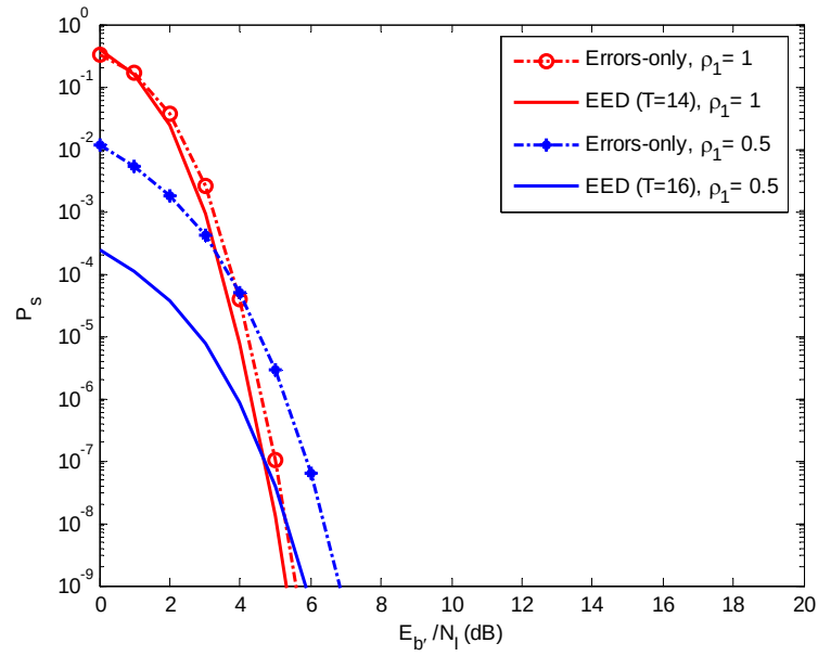
Figure 77. Probability of symbol error of a JTIDS/Link-16-type waveform for the double-pulse structure with PSI in both AWGN and PNI when the signal is transmitted over a slow, flat Nakagami fading channel where m = 30 and E_{b'}/N_0 = 15 dB: EED versus errors-only RS decoding.
