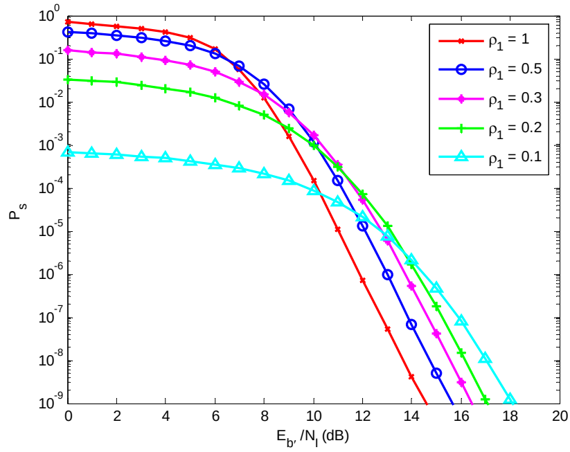
Figure 45. Probability of symbol error of a JTIDS/Link-16-type waveform for the single-pulse structure in both AWGN and PNI transmitted over a slow, flat Nakagami fading channel where m = 5 and E_b/N_0 = 10 dB.
