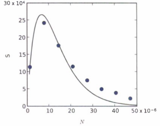
FIG. 5. (Color online) The maximum value of the interference signal as a function of number of atoms in the trap. The solid curve is Eq. (38) and the dots were extracted from a DSMC calculation.
