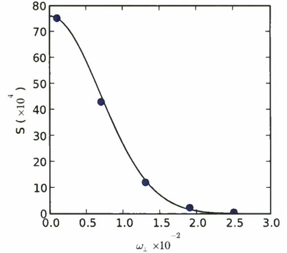
FIG. 3. (Color online) The maximum value of the interference signal as a function of perpendicular trapping frequency. The solid curve is found using Eq. (38) and the dots were extracted from a DSMC calculation.
