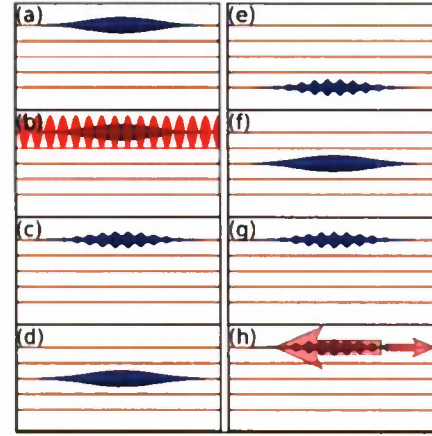
FIG. 1. (Color online) A schematic of the interferometer cycle. (a) The cold gas is loaded into a cigar-shaped trap, created with the upper most horizontal wire. (b) The atomic cloud is illuminated with a standing wave laser field. (c) After the laser pulse, a density modulation appears across the cloud. (d) The density modulation disappears and the trap is moved downwards by cycling the current in the wires. (e) The trap is above the bottom wire at a half period of the parallel trap and the density modulation reappears across the cloud. (f) The trap is moved upward and the density modulation disappears. (g) The trap reaches the top wire at one trap period of the parallel trap and the density modulation reappears for a second time. (h) A probe pulse is reflected off of the cloud.
