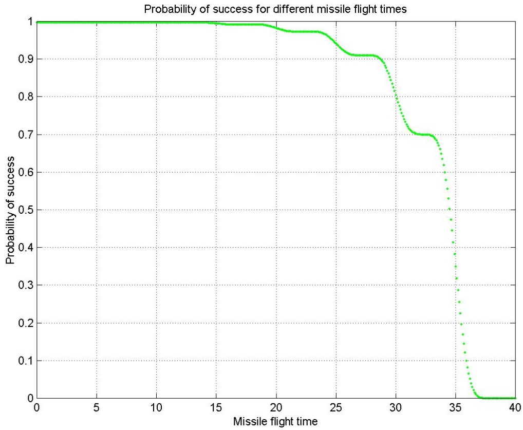
Figure 1. Probability of success for different missile flight times*
