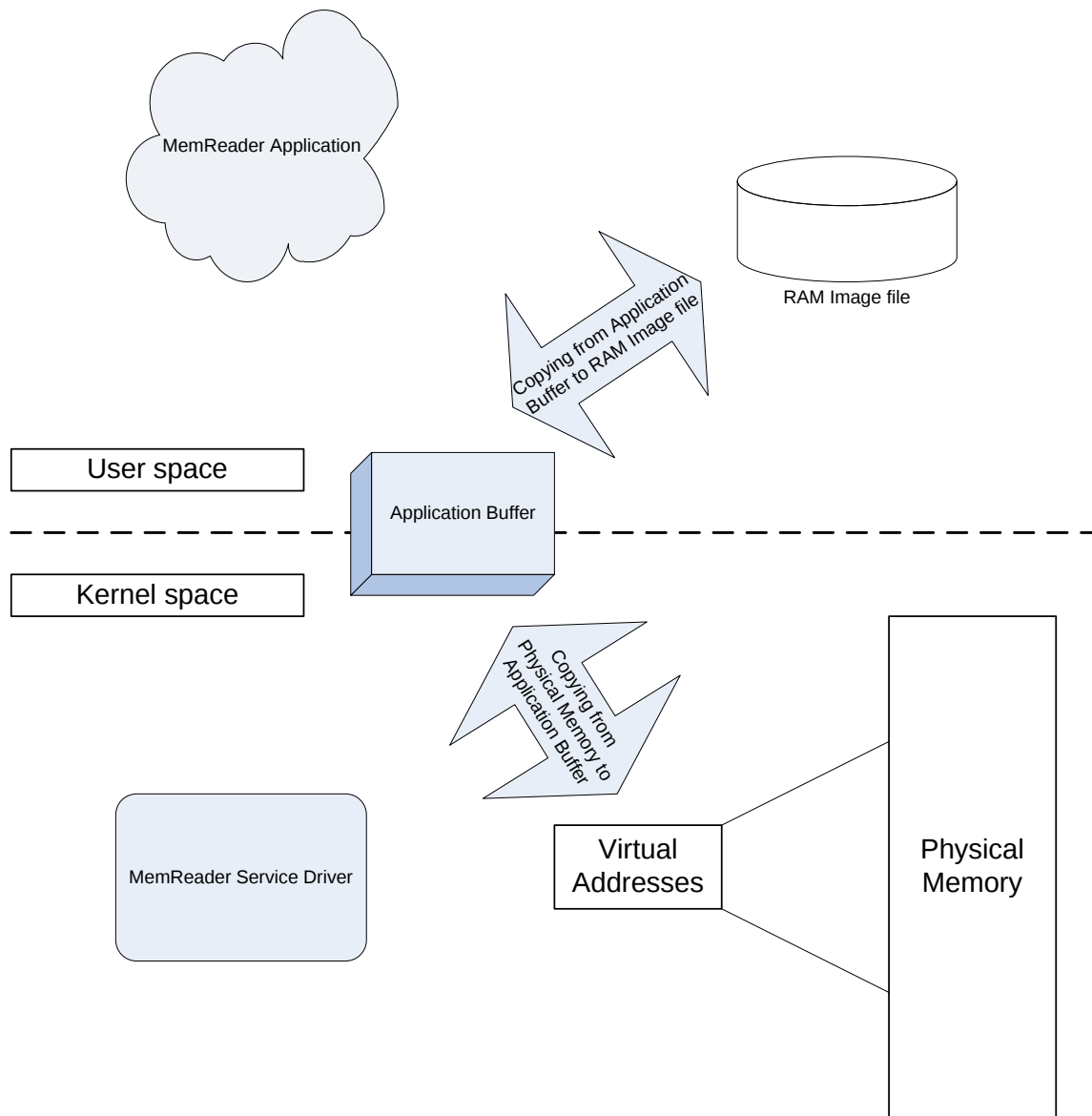
Figure 1. Graphical Representation of MemReader Application and Driver
