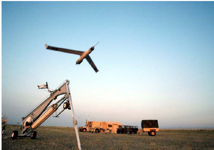
Figure 12. ScanEagle Launched Using A Catapult [From 7].
