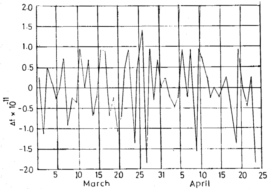
Fig.5 Frequency offset vs Hp 5061A Cs
