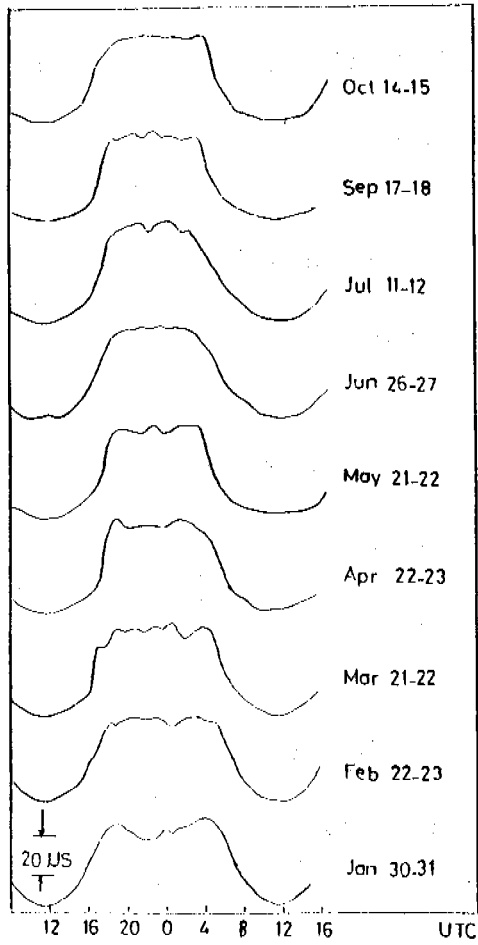
Fig. 3 30-hour diurnal phase variation Liberia-Cairo, 1985
