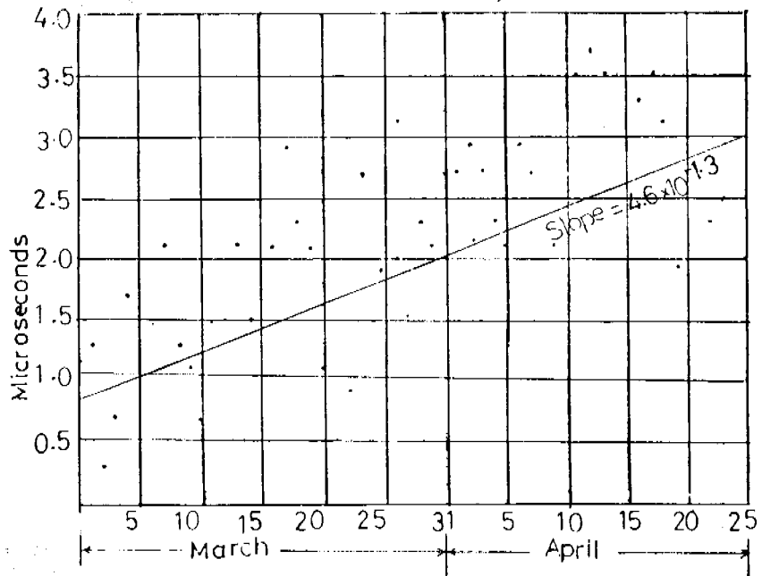
Fig. 4. Phase record of Liberia at Cairo, Egypt.
