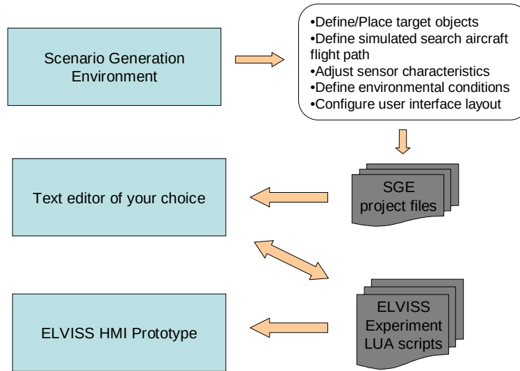
Figure 18. AIMSSim experiment development process when it involves the SGE
