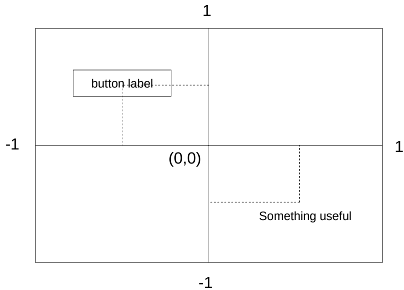
Figure 13. Example dialog screen, also shows coordinate system
