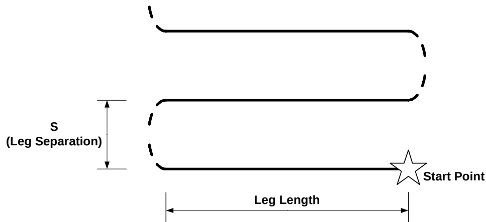
Figure 26. Creeping Line Ahead Parameters
