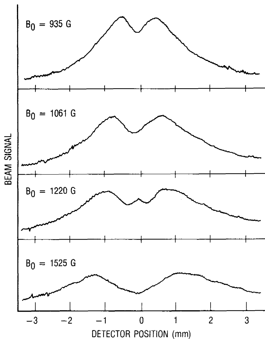
Figure 17: Rubidium atomic beam intensity profiles after deflection in the "two-wire" field magnet; fields are given in gauss. The central features at B_0 = 1220 \text{ G} is the signature of the m = -1 states, which have zero effective magnetic moment at that field strength.
