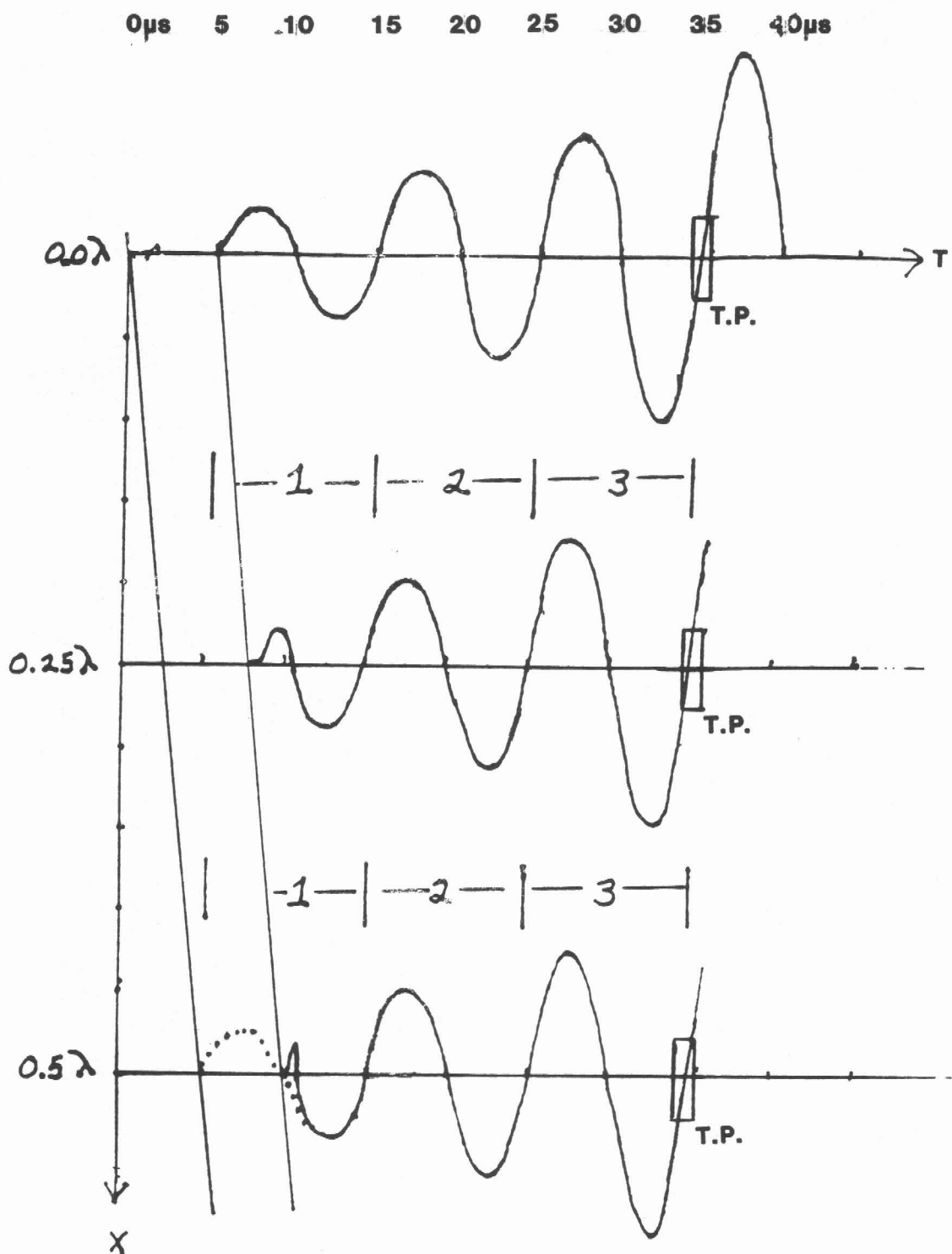
FIG. 22 Note compressed first positive half-cycle that radiates as low level delta-function spike
